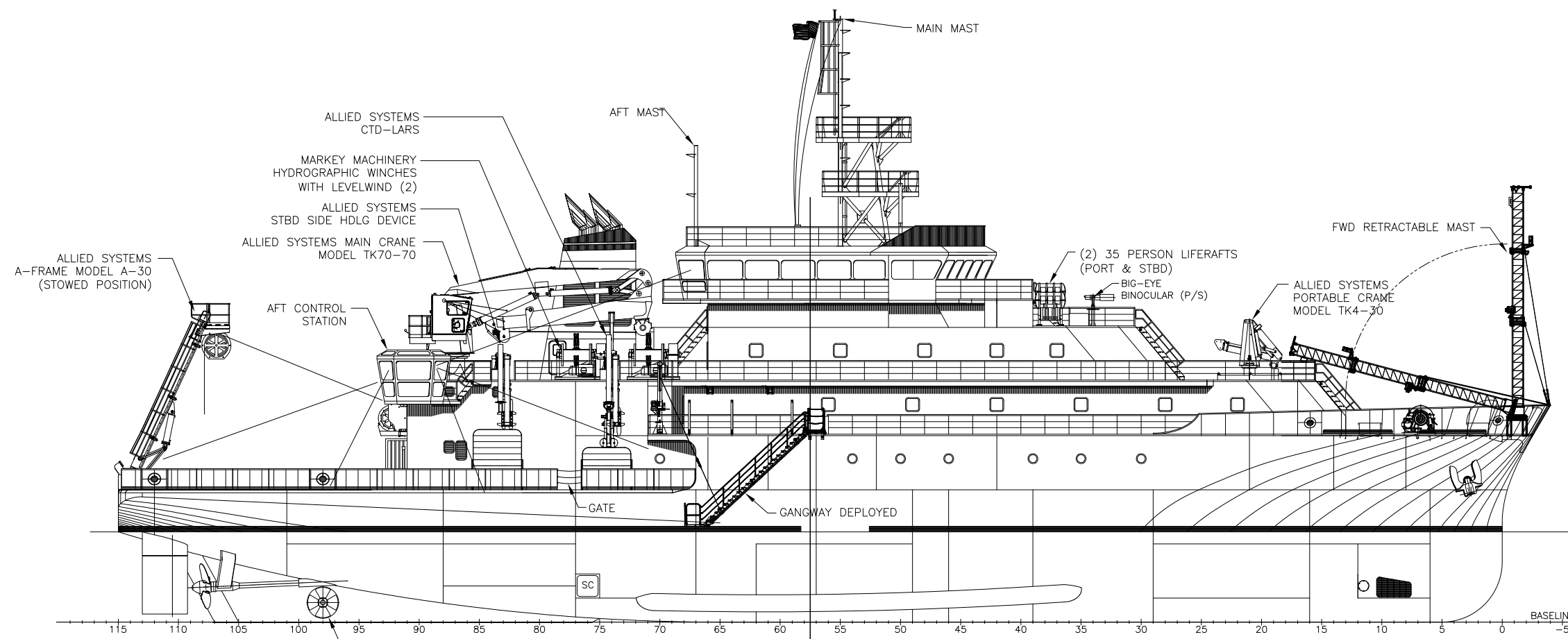
OUTBOARD PROFILE
