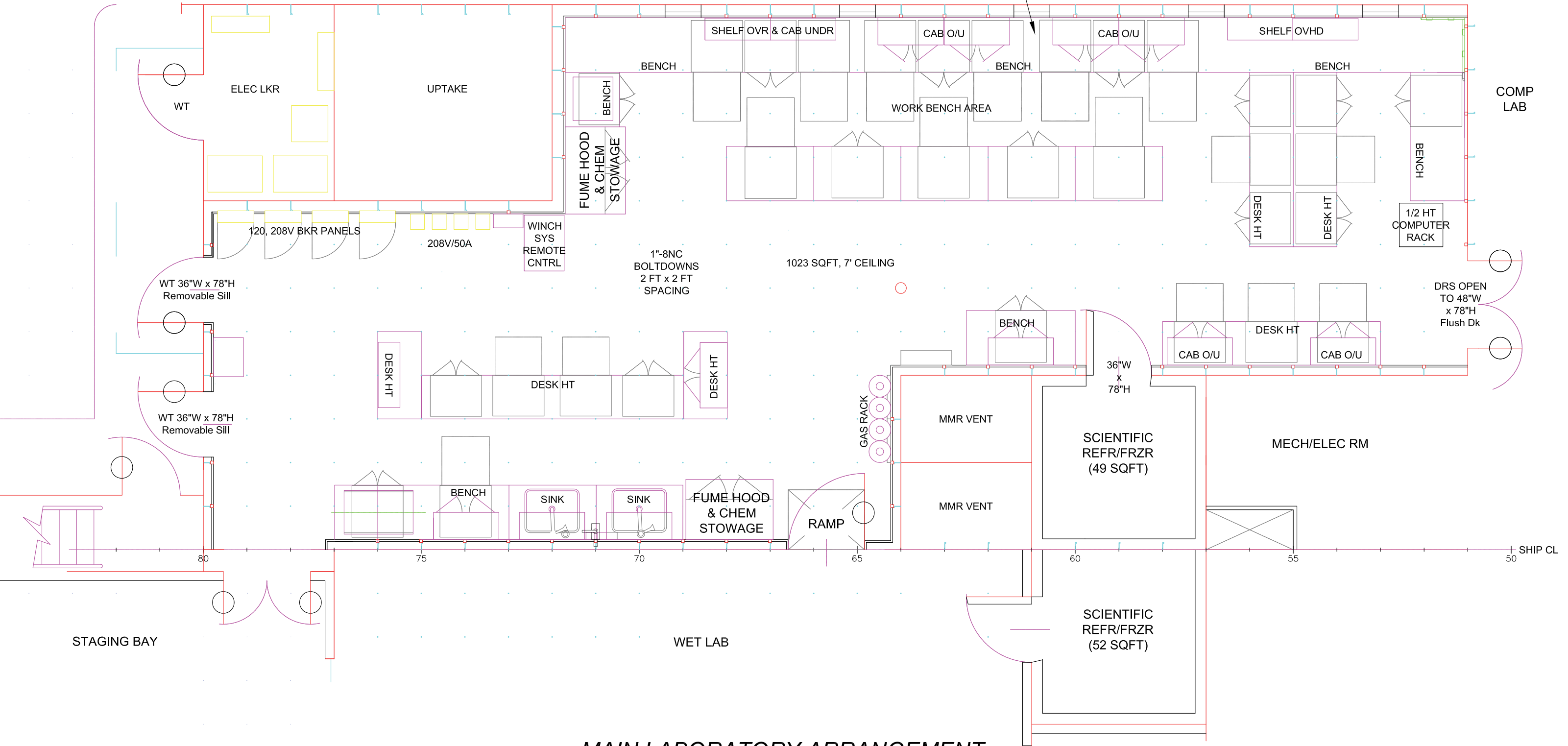
MAIN LABORATORY ARRANGEMENT
