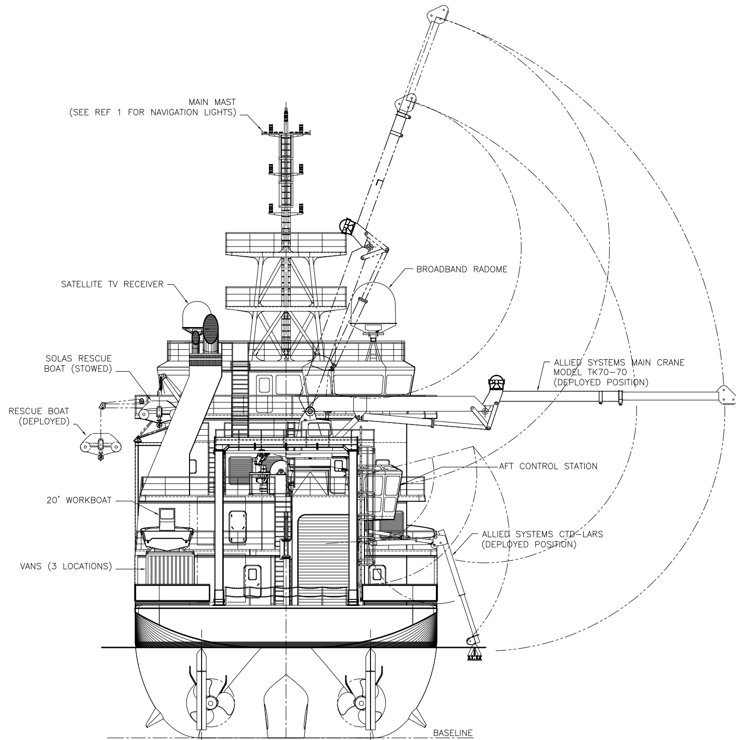
STERN VIEW
