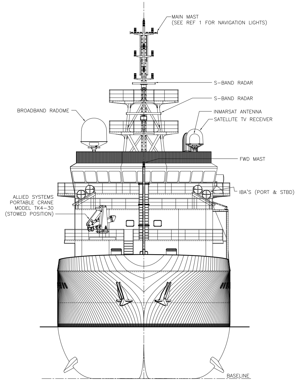
BOW VIEW
