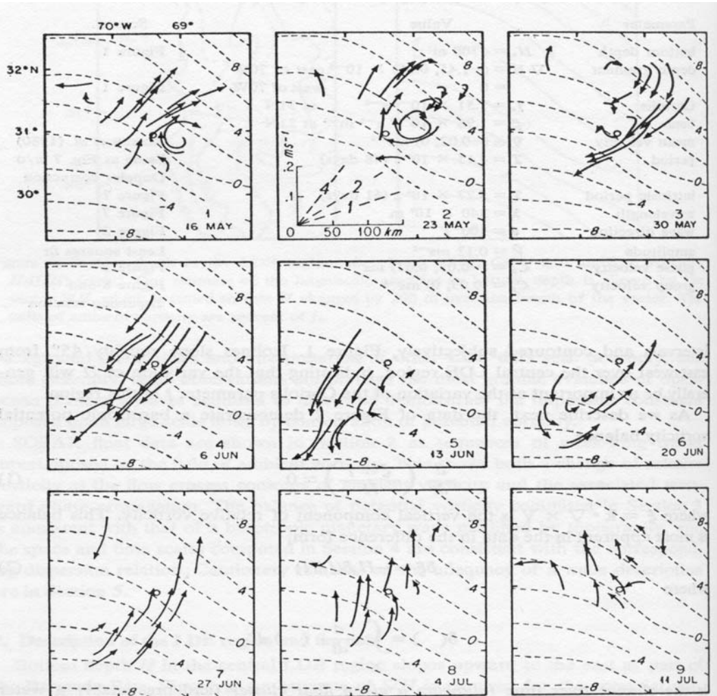
Figure 2. Week-long float trajectories superimposed over ambient vorticity contours. These data have been smoothed with a two-day Gaussian taper to remove tidal and inertial energy. The open circle at 31.0N, 69.5W marks the location of the LDE central mooring. The panel number and the beginning date are noted at lower right of each panel. Speed, distance and a relative vorticity scale are in Panel 2. Units of relative vorticity are percent of f_* (same as the ambient vorticity contours).
