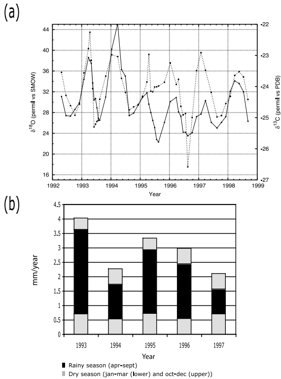
Fig. 6. (a) High-resolution \delta^{18}\text{O} (solid) and \delta^{13}\text{C} (dashed) records of the P. neriifolius DIN99W from the Doi Inthanon National Park, northern Thailand. Data are fit to an age model based on the time of wounding (10/92) and time of cutting (02/99) of the wedge section as well as seasonal changes in RH (see text for details). The number of well-defined isotopic cycles corresponds to the number of years elapsed between wounding and cutting of the sample. The data illustrate how high-resolution isotopic records may be used as independent chronometers of tropical climate history. (b) Growth rate estimates based on isotopic age model shown in (a).
