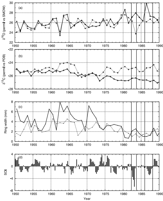
Fig. 4. (a) Comparison of the \delta^{18}\text{O} records of SA02A (solid) and SA06A (dashed) with correlation coefficients r(1950-1990)=0.40 ( P=0.005 ) and r(1950-1980)=0.69 ( P<0.0001 ). Based on the age and growth rates of the two trees, we observe that the younger SA02A tree appears more sensitive to large El Niño events than SA06A as it probably relies more heavily on seasonal recharges in soil water from rainfall. (b) Same as in (a) but for the \delta^{13}\text{C} records. (c) Ring width comparison between SA02A (dashed) and SA06A (solid) with correlation r=0.54 ( P=0.0002 ) over the period from 1950 to 1990. For the first 30 years of the record, SA02A has faster growth rates than SA06A as it is much younger (growth curve not removed). A decline in the growth rates of both trees (although more drastic for SA02A) is apparent after the mid-1970s. (d) Seasonally averaged SOI (standardized Tahiti – standardized Darwin) [65]. Low (high) values indicate El Niño (La Niña) events. Vertical solid lines bracket the 1982–1983 and 1986–1987 El Niño events.
