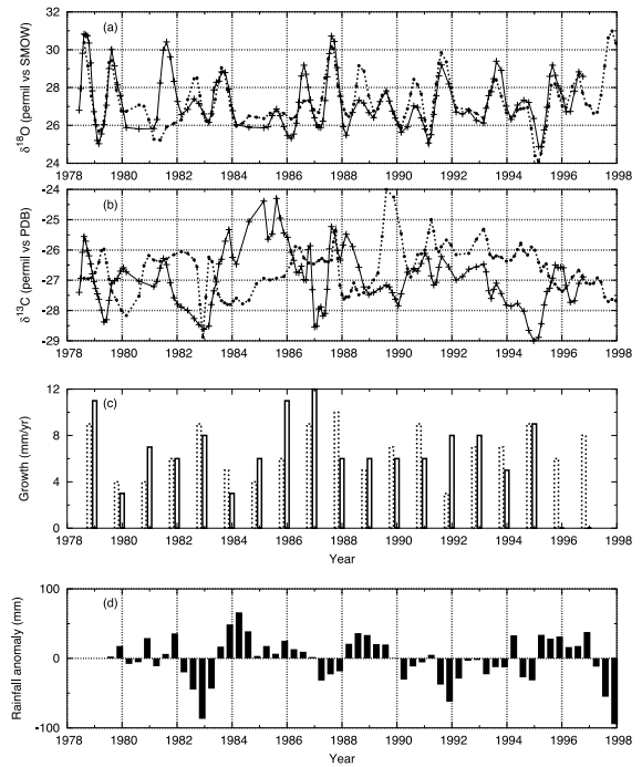
Fig. 5. (a) \delta^{18}\text{O} comparison between Suar1 (dashed) and Suar3 (solid). The amplitudes of the oxygen isotopic variations are remarkably similar suggesting that the trees are recording an environmental forcing that was common to both ( r=0.68 , P<0.0001 ). The chronology of the ringless trees is based on estimated radiocarbon age model (see text for details). (b) Same as in (a) but for \delta^{13}\text{C} . (c) Growth rate estimates for Suar1 (dashed) and Suar3 (solid) obtained using the measured radiocarbon ages. (d) Seasonal precipitation anomalies (FMAM, JJAS, ONDJ) for the region 109–124°E and 11°30'S and 4°30'N [40].
