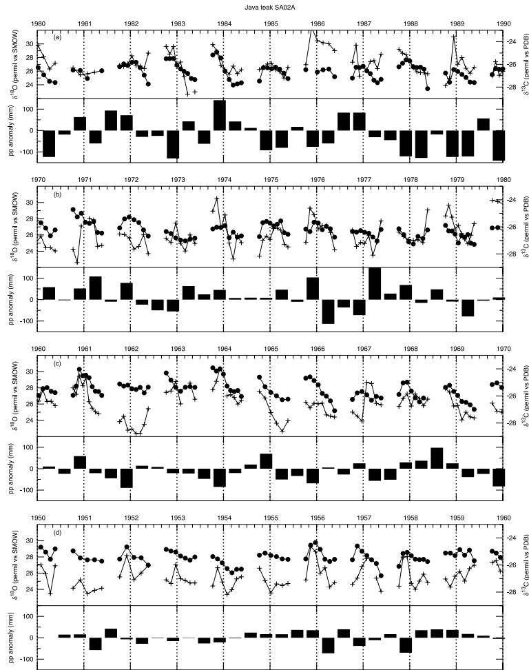
Fig. 2. Comparison of the \delta^{18}\text{O} (crosses) with \delta^{13}\text{C} (filled circles) records for the teak SA02A. Sub-annual samples within individual rings represent equivalent growth increments but may not reflect equivalent time increments as growth rates are likely to vary throughout the year. The age model is based on the fact that most of the teak growth in Indonesia occurs during the rainy season, from October to May [48]. Seasonal precipitation anomalies (FMAM, JJAS, ONDJ) centered on the region 111^\circ\text{E} and 7^\circ\text{S} [64].
