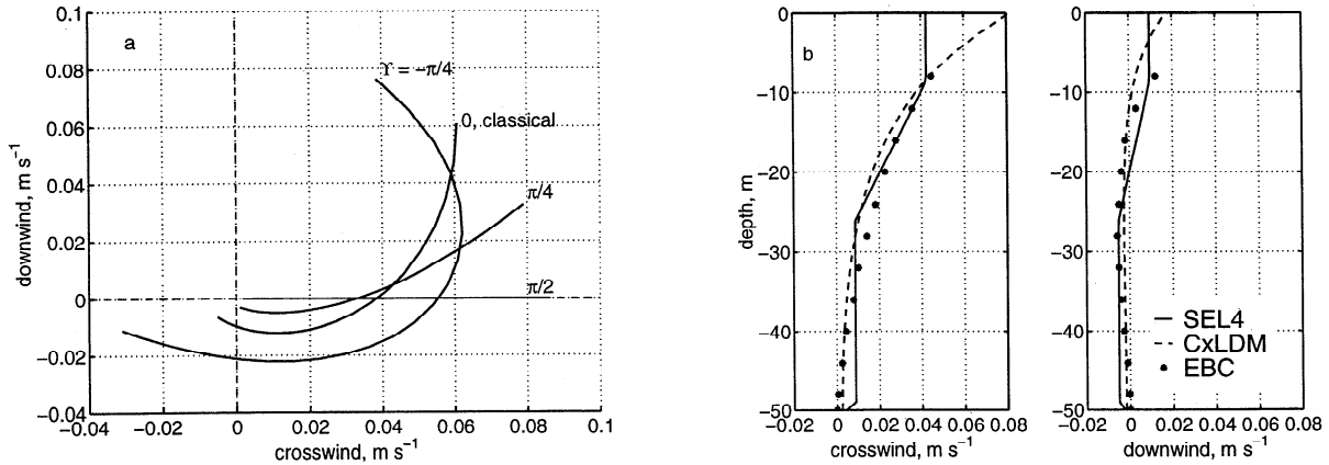
Figure 18. Solutions of the C x LDM with external parameters set to EBC values. (a) Solutions for various \gamma . A classical spiral has \gamma = 0 and stress parallel to shear, while \gamma > 0 gives a stress to the left of the shear and flatter spirals. (b) Ekman layer currents computed by the SEL4 and C x LDM solutions. The two solutions are generally similar, except in the upper 5 m of the water column, where the crosswind component of C x LDM is considerably larger.
