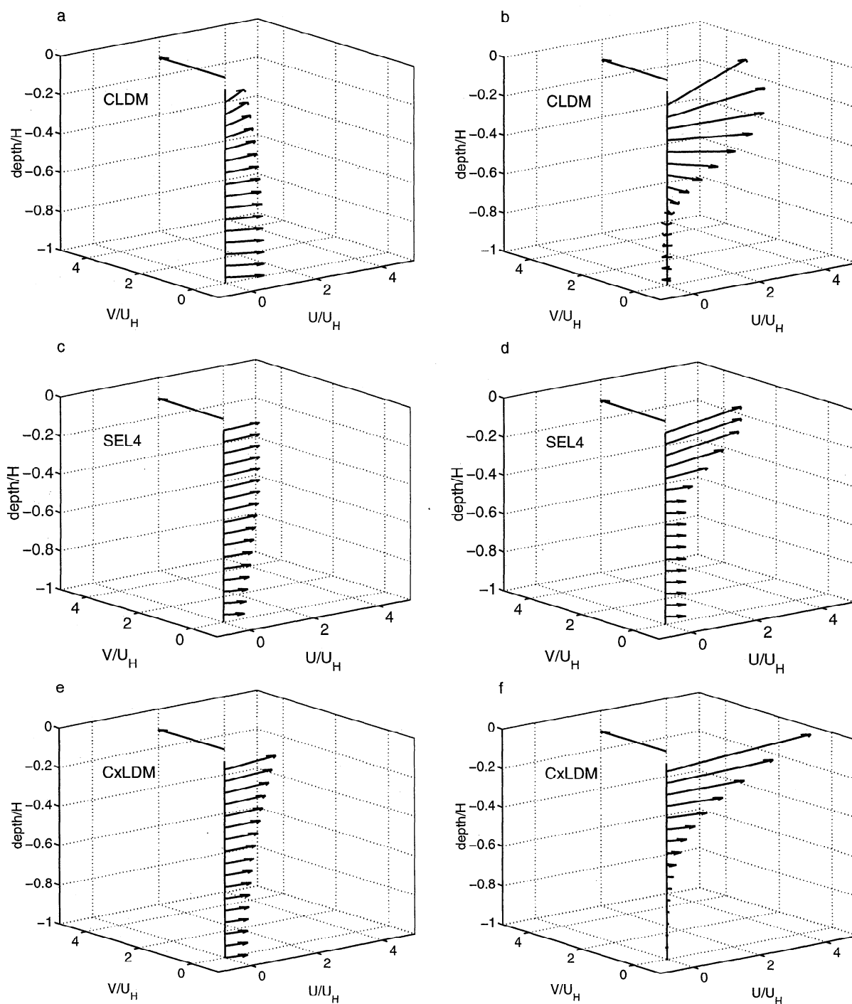
Figure 3. Ekman layer current profiles computed by three different models for midlatitude conditions, latitude = 37^\circ , \tau_w = 0.08 \text{ Pa} , and H = 50 \text{ m} , which give a neutral velocity scale U_H = 0.022 \text{ m s}^{-1} , (a, b) from the Classical Laminar Diffusion Model (CLDM); (c, d) from the four-layer stratified Ekman layer model (SEL4) developed in section 5; (e, f) from the complex laminar diffusion model ( C_X LDM) developed in section 6. The CLDM solutions had K = 750 \times 10^{-4} and 50 \times 10^{-4} \text{ m}^2 \text{ s}^{-1} , which correspond to \alpha = 1.2 and 4.6 (Figures 3a and 3b, respectively). The SEL4 and C_X LDM solutions had the same wind stress and Q = 100 and 1200 \text{ W m}^{-2} (Figures 3c and 3d and 3e and 3f, respectively), so that \alpha corresponds to the CLDM solutions at the top.
