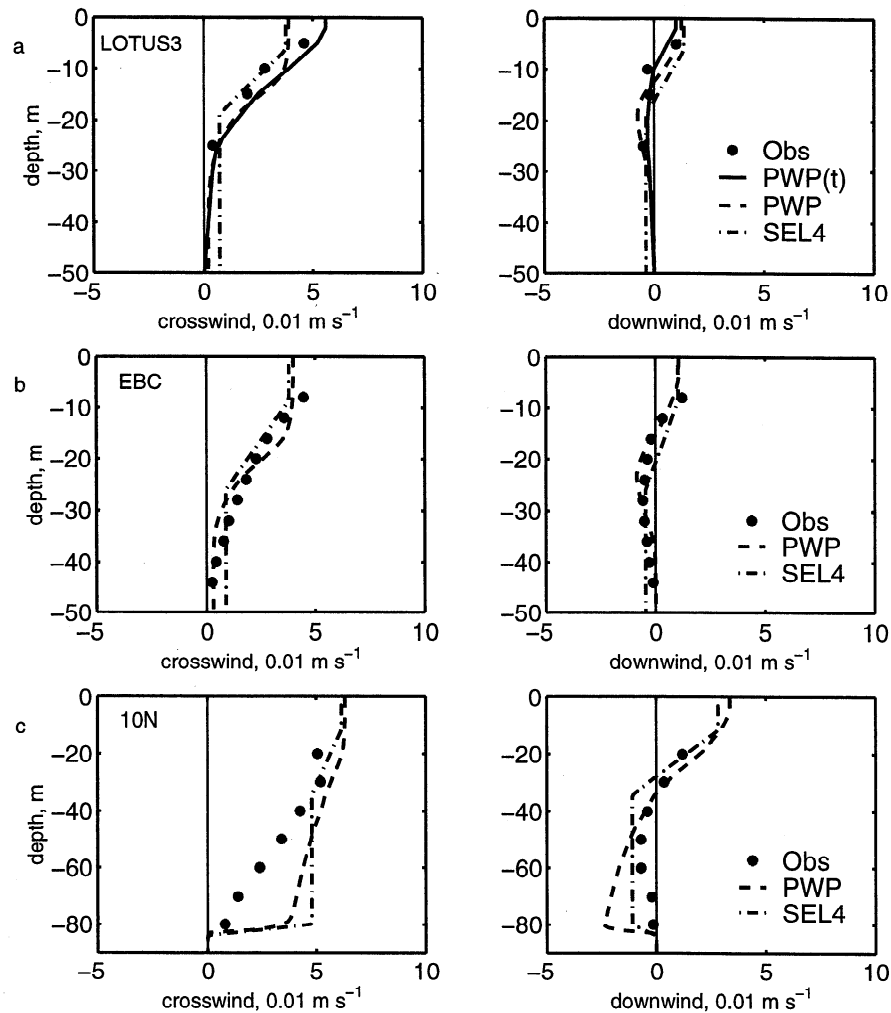
Figure 15. Comparisons of the SEL4 solution (dash-dotted lines) with the PWP numerical solution (dashed lines), and in the LOTUS3 case only, with the PWP numerical model run using the hourly surface fluxes (solid line) for (a) LOTUS3, (b) EBC, and (c) 10°N. The solid dots are the observations.
