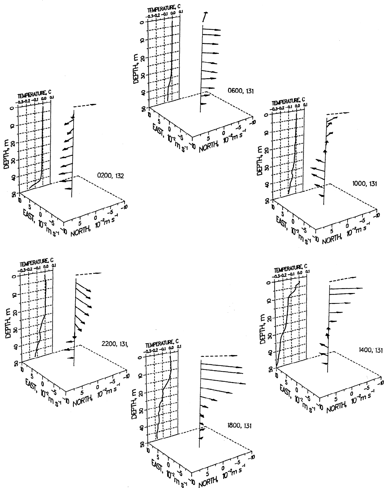
Figure 7. An observed diurnal cycle of temperature and current from Price et al. [1986]. Currents were measured by vector-measuring current meters, smoothed over 30 min at a given depth and referenced to 50 m depth. Temperature was measured by conductivity-temperature-depth (CTD) profilers and referenced to the sea surface. The uppermost dashed vector shows the wind stress direction.
