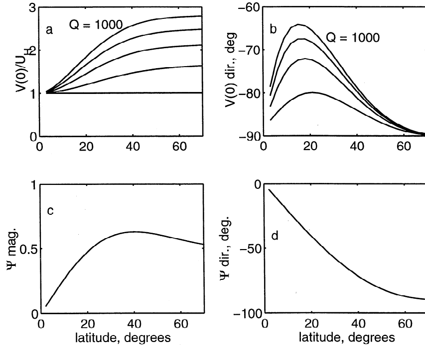
Figure 16. Parameter dependence of the SEL2 surface current (same as SEL4). (a) Speed of the surface current normalized by the neutral velocity scale for \tau_w = 0.1 \text{ Pa} , H = 50 \text{ m} (held fixed), and Q = 250, 500, 750 , or 1000 \text{ W m}^{-2} and as a function of latitude. Speeds greater than 1 show some effect of diurnal cycling. (b) The direction of the surface current with respect to the wind stress (negative direction is to the right of the wind stress). The surface current is at nearly right angles to the wind stress for conditions of very low heating, in which case there is no effect of diurnal cycling, and also at very low and very high latitudes, regardless of the heating. (c) Amplitude and (d) phase of \Psi . Recall that the time-averaged shear due to diurnal cycling is proportional to \Psi .
