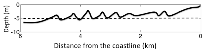
Bottom Profile at el Cuyo (adapted from Liceaga-Correa et al., 2012)
