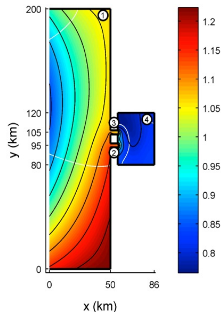
Figure 1: Co-tidal chart for an example of a double inlet system with 4 compartments. Elevation amplitudes are in meters, co-phase lines ( white ) have intervals of 30^\circ and co-range lines ( black ) have intervals of 5 cm. The inlet widths and lengths are 3 km and 6 km respectively.
