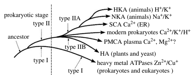
Figure 12. Evolution of the metal ion pumps. The variety of Ca^{2+} pumps rose with the coming of eukaryotes and those for Na^+/K^+ rose with the evolution of animals with nerves. Heavy metal ion pumps have been necessary from very primitive cell times.
