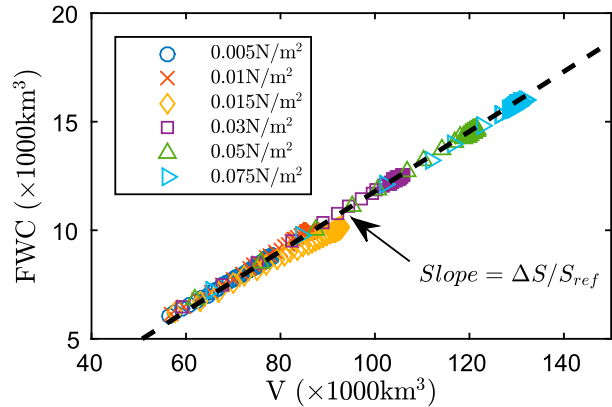
FIG. 5. Freshwater volume and freshwater content plotted against each for the spinup time series of different numerical model experiments. Dashed line shows a slope of \Delta S/S_{\text{ref}} supporting Eq. (31).
