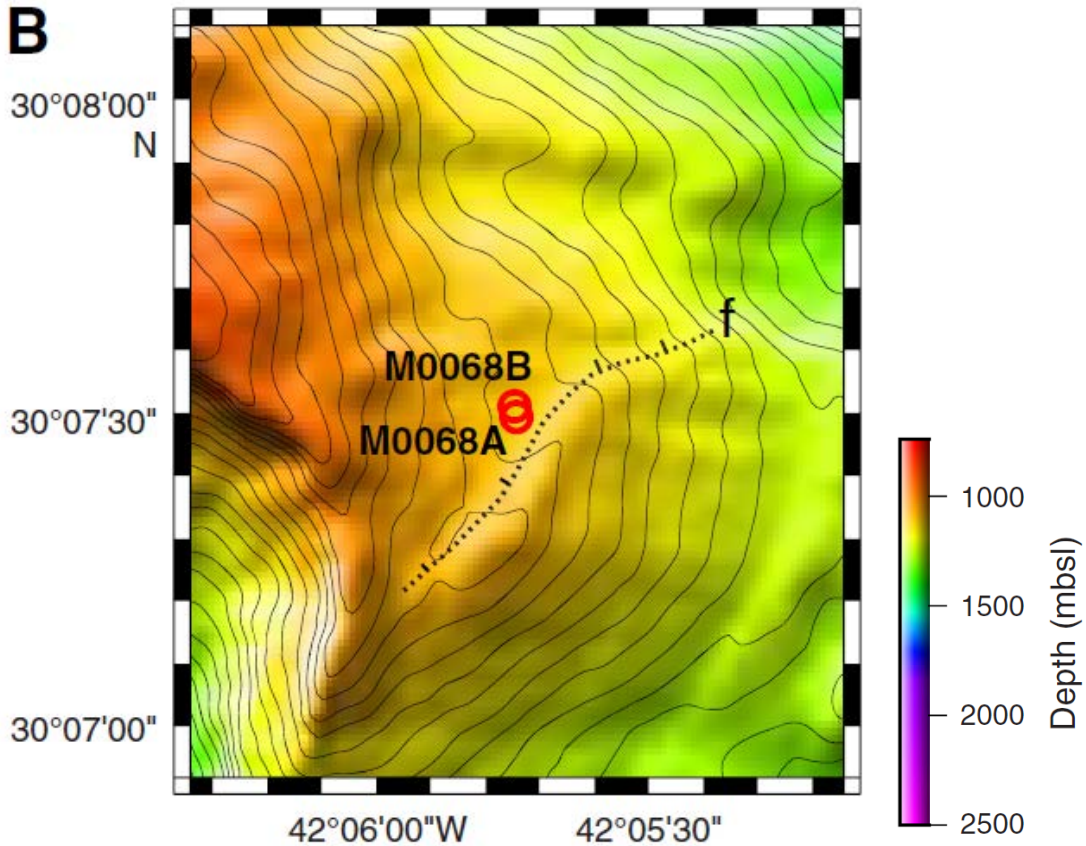
Maps of Expedition 357 Boreholes. Contour interval = 20 meters
