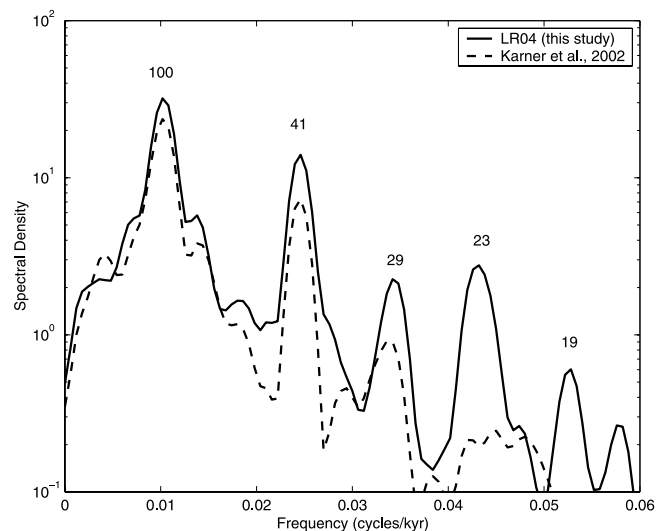
Figure 12. The spectral density of benthic \delta^{18}\text{O} over the last 860 kyr in the LR04 stack (solid line) and the minimally tuned tropical stack of Karner et al. [2002] (dashed line). Spectral analysis is performed using Blackman-Tukey analysis with 500 lags on 860 values. (The peak at 29 kyr is commonly observed and is thought to be a nonlinear climate response [e.g., Huybers and Wunsch , 2004].)
