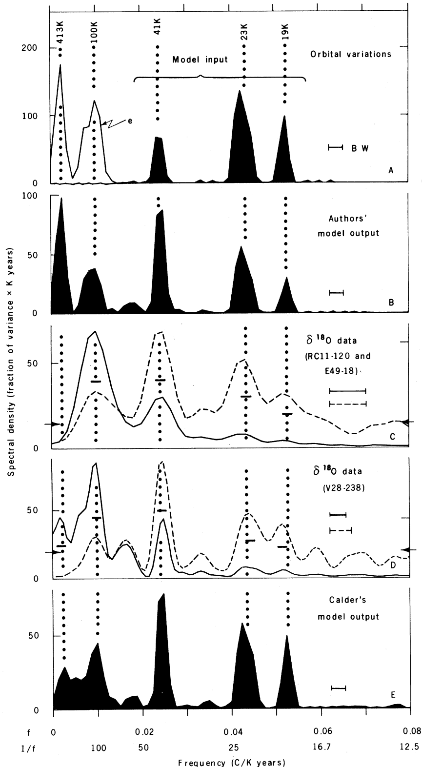
Fig. 9. Spectral density as a function of frequency f (cycles per 1000 years). Climatic spectra are compared with input spectra and output spectra of two climate-response models (80). (A) Solid peaks are the spectrum of the input to our optimum model. Open peaks are the spectrum of variations in eccentricity calculated from data of Berger (19). The dominant periods of these orbital variations, calculated by Berger (22), are indicated in thousands of years and by dotted vertical lines. (B) Spectrum of the output of our optimum model. Note the low-frequency peaks not found in the model input. (C) Solid line shows spectrum of variations in \delta^{18}\text{O} from a 468,000-year record in the southern Indian Ocean. Dashed line shows spectrum of same data after prewhitening with a first-difference filter to emphasize details in the higher frequencies. Data are from Hays et al. (5), with the spectrum calculated on their TUNE-UP time scale. (D) Solid line shows spectrum of variations in \delta^{18}\text{O} from a 730,000-year core record in the Pacific Ocean. Dashed line shows spectrum of the same data after prewhitening with a first-difference filter to emphasize details in the higher frequencies. Isotopic data are from Shackleton and Opdyke (7). Time scale and unprewhitened spectrum are from Kominz et al. (8, 9). (E) Spectrum of the output of a response model due to Calder (59). Note the low-frequency peaks not found in this model's orbital input, whose spectrum is almost identical to that shown by solid peaks in (A). Data for (A), (B), and (E) span approximately the last million years. The bandwidth (BW) of each spectrum is indicated by horizontal lines. Horizontal bars within peaks in (C) and (D) are the lower bounds of one-sided 90 percent confidence intervals attached to estimates of peak heights. For each prewhitened spectrum in (C) and (D), the level of a red-noise continuum is marked by arrows.
