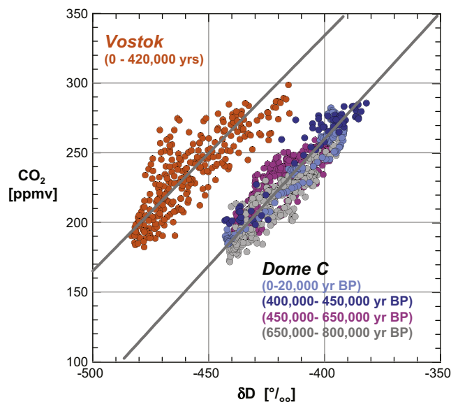
Fig. 2. CO 2 concentrations vs. δD as shown in Fig. 1. Respective δD values for each CO 2 value were calculated by linear age interpolation of the δD values in 500 yr resolution to ensure a temporal resolution comparable to the one for glacial CO 2 data. Straight lines represent two-sided linear regressions over the entire data sets. Note, that EDC CO 2 concentrations prior to 450,000 yr BP do not span the whole CO 2 range but show a similar linear relationship with temperature. Only CO 2 data during MIS 16–18 are systematically reduced by about 10 ppmv.
