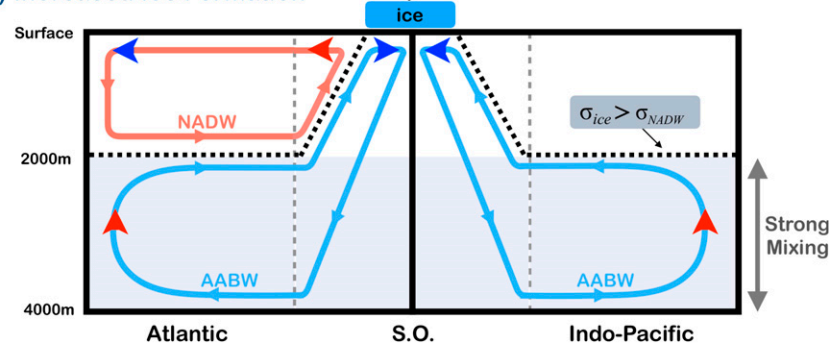
FIG. 1. Schematic of the meridional overturning circulation for (a) the present-day climate, (b) increased permanent Antarctic sea ice extent, and (c) increased Antarctic sea ice formation rate. Water masses belonging to the upper cell are represented by red lines, whereas those belonging to the abyssal cell are represented by blue lines. Red and blue arrows represent water mass transformation (lighter and denser, respectively) occurring through surface fluxes in the mixed layer or through diapycnal mixing in the ocean interior. In each panel, the isopycnal outcropping at the ice edge \sigma_{ice} is represented by a black dashed line. The deepest density class of NADW is referred to as \sigma_{NADW} .
