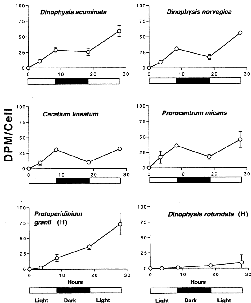
Fig. 1. Expt 1, water from the Tjörnö Strait, October 1992. ^{14}\text{C} uptake by different dinoflagellate species after exposure of a natural plankton community to light and dark incubations. Cells were isolated under the microscope and placed in scintillation vials. Each point is the mean \pm SD of 4 scintillation vials, each vial containing 15 to 50 cells. H: species that are completely heterotrophic
