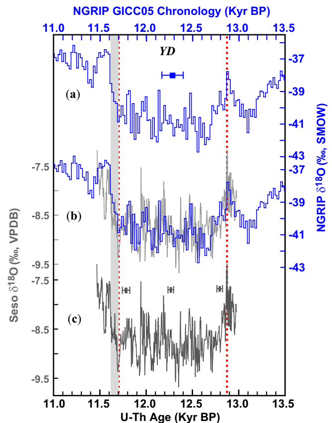
Fig. 1. Comparison between Greenland NGRIP ice-core and Sesó speleothem \delta^{18}\text{O} records. (A, C) Greenland NGRIP (25) and Sesó speleothem \delta^{18}\text{O} records (this study), respectively. (B) Comparison between NGRIP (blue) and Sesó (gray) \delta^{18}\text{O} records. The error bars show the typical age error of each YD record (color-coded). The two vertical red dashed lines depict the initial onset (the abrupt drop at \sim 12,870 \pm 30 B.P.) and initial termination (initiated at \sim 11,700 \pm 40 B.P.) of the YD based on correlation of distinct features at subcentennial precision. The gray bar shows the YD termination excursion from \sim 11,700 to \sim 11,610 B.P. Kyr BP, 1 \times 10^3 B.P.
