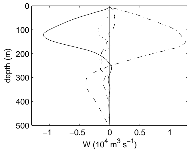
FIG. 5. Vertical mass transport averaged between 20 km and 30 km longitude between days 3 and 10. solid line: cooling decays offshore; dot-dashed line: cooling increases offshore; dashed line: uniform cooling; dotted line: insulated within 3 km of the southern boundary.
