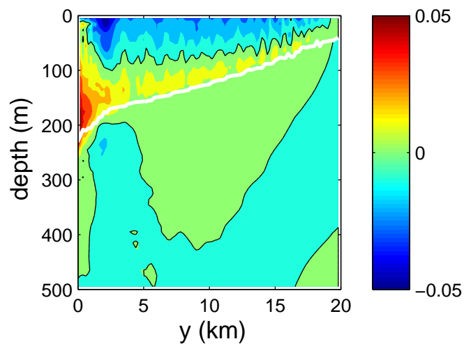
FIG. 8. The difference in zonal velocity averaged between 20 km and 30 km longitude between a calculation with surface cooling and a calculation with no surface forcing ( \text{m s}^{-1} ). The zero contour is in black and the mixed layer depth is given by the white line.
