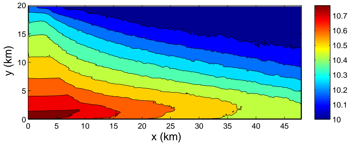
FIG. 1. Temperature at 45 m depth averaged between days 2 and 6 for uniform cooling of 500 \text{ W m}^{-2} and a velocity field that decays offshore.
