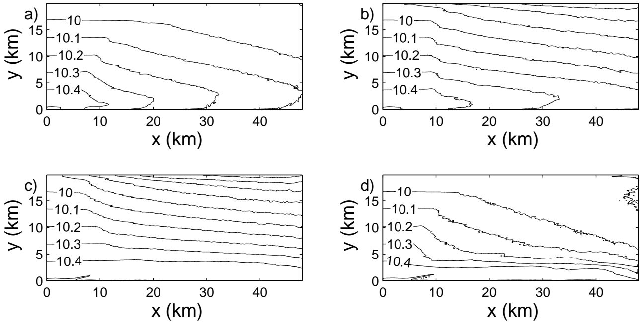
FIG. 4. Temperature at 45 m depth averaged between days 3 and 10 for cases with uniform horizontal velocity at each depth. Heat flux: a) linearly decays from 1000 \text{ W m}^{-2} at y = 0 to 0 at y = 20 \text{ km} ; b) spatially uniform at 500 \text{ W m}^{-2} ; c) linearly increases from 0 at y = 0 to 1000 \text{ W m}^{-2} at y = 20 \text{ km} ; d) linearly decays from 1176 \text{ W m}^{-2} at y = 3 \text{ km} to 0 at y = 20 \text{ km} .
