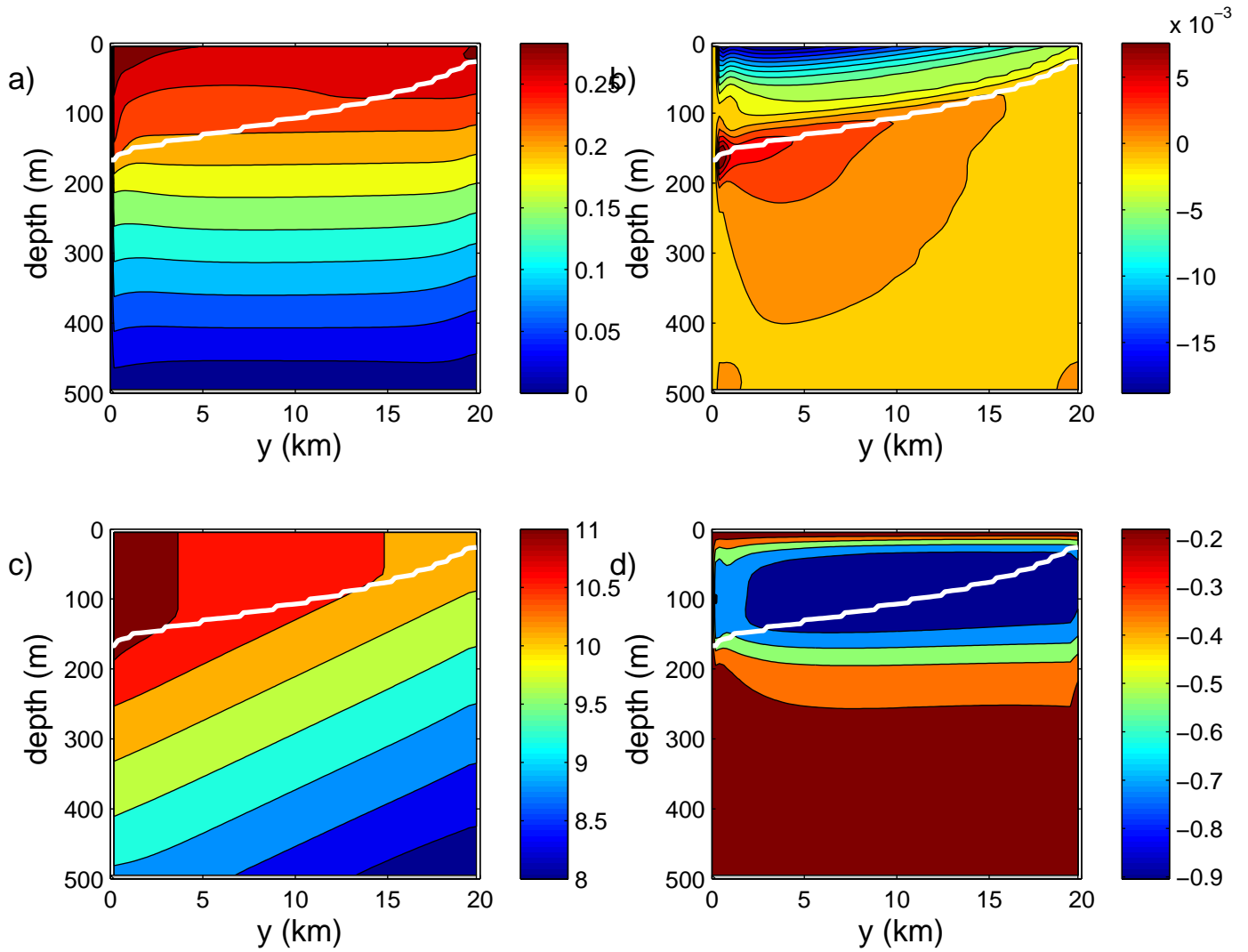
FIG. 12. Vertical section of a) zonal velocity (m/s); b) meridional velocity (m/s); c) temperature ( ^{\circ}\text{C} ); d) transport streamfunction ( 10^4 \text{ m}^3 \text{ s}^{-1} ) averaged between 20 km and 30 km longitude between days 3 and 10 for the case with hydrostatic physics, free-slip boundary conditions, and viscosity and diffusivity of 5 \text{ m}^2 \text{ s}^{-1} . The inflow velocity is uniform and the surface cooling decays from 1000 \text{ W m}^{-2} at y = 0 to zero at y = 20 km. The white line indicates the average mixed layer depth.
