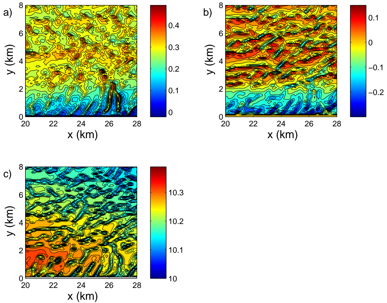
FIG. 9. a) Zonal velocity, b) meridional velocity at 5 m depth and c) temperature ( ^{\circ}\text{C} ) at 15 m depth on day 10 (velocity in \text{m s}^{-1} ).
