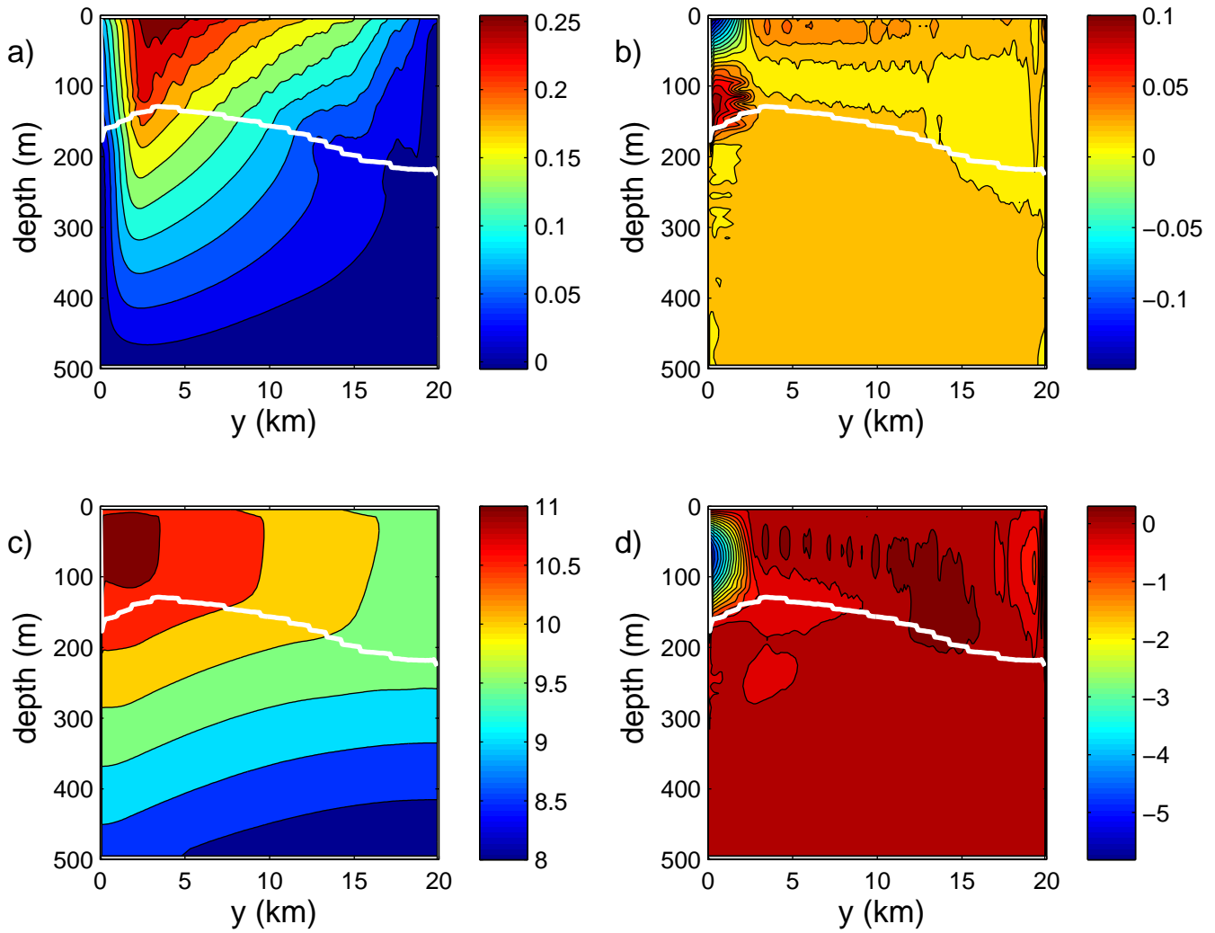
FIG. 2. Vertical section of a) zonal velocity (m/s); b) meridional velocity (m/s); c) temperature (C); d) transport streamfunction ( 10^4 m^3 s^{-1} ) averaged between 20 km and 30 km longitude between days 2 and 6. The white line indicates the average mixed layer depth.
