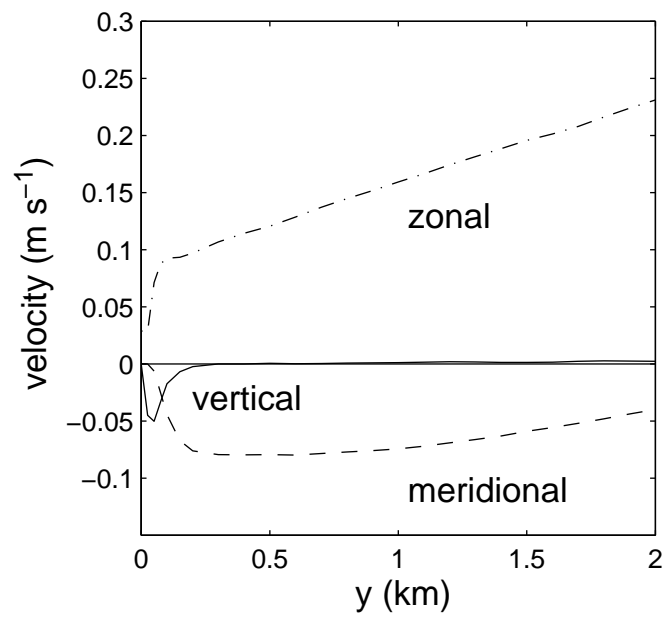
FIG. 10. The mean horizontal and vertical velocities near the southern boundary at 100 m depth from the calculation with enhanced meridional resolution near the boundary.
