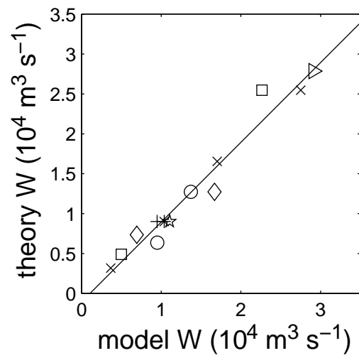
FIG. 11. Comparison of the net downwelling rate per unit along-boundary distance calculated from the model and that predicted by the theory (9). Each symbol corresponds to a different calculation in which the cooling rate, vertical stratification, horizontal stratification, Coriolis parameter, or basin depth were varied (see Table 1 for a summary).
