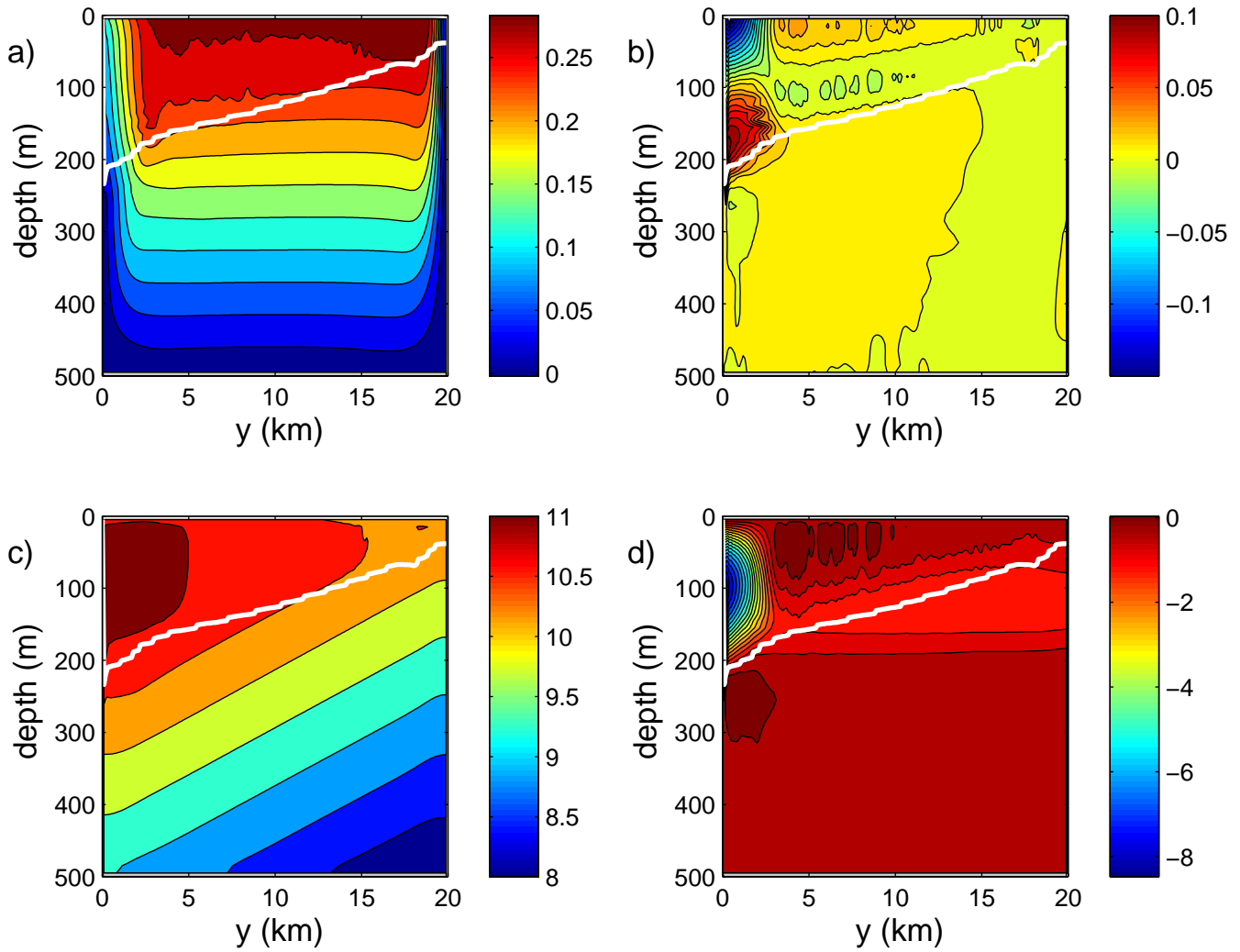
FIG. 7. Vertical section of a) zonal velocity (m/s); b) meridional velocity (m/s); c) temperature ( ^{\circ}\text{C} ); d) transport streamfunction ( 10^4 \text{ m}^3 \text{ s}^{-1} ) averaged between 20 km and 30 km longitude between days 3 and 10 for the case with uniform inflow velocity and cooling that decays to zero at y = 20 \text{ km} . The white line indicates the average mixed layer depth.
