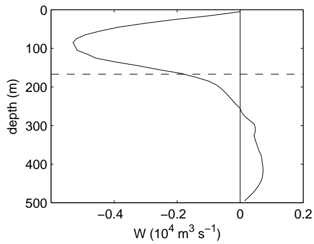
FIG. 3. Vertical mass transport averaged between 20 km and 30 km longitude between days 2 and 6. The average mixed layer depth is indicated by the dashed line.
