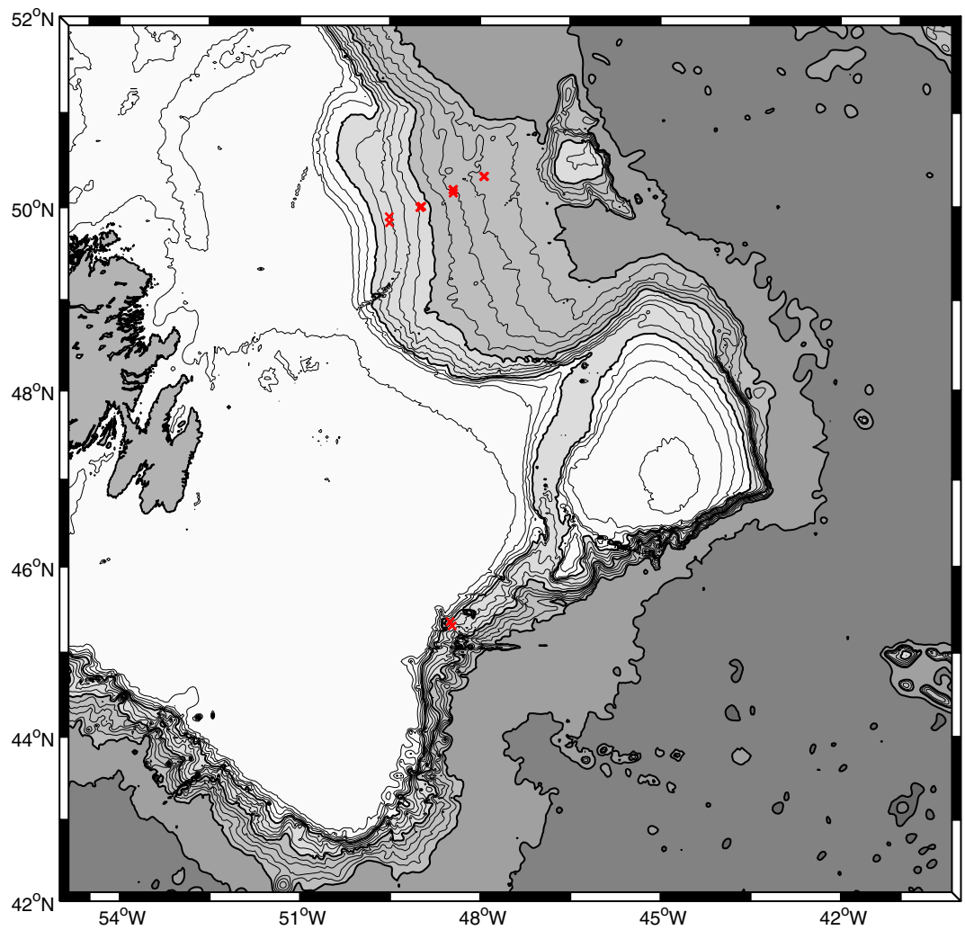
Float Launch Locations. Includes two cruises on the Bonavista Line, and test floats released east of Grand Banks. Thick black lines are 100 m contours, and follow shaded bathymetry; Thin lines are every 200 meters, down to 3000 meters depth.
