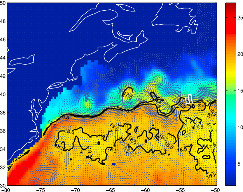
SST & surface velocity for Feb 22, 2007
