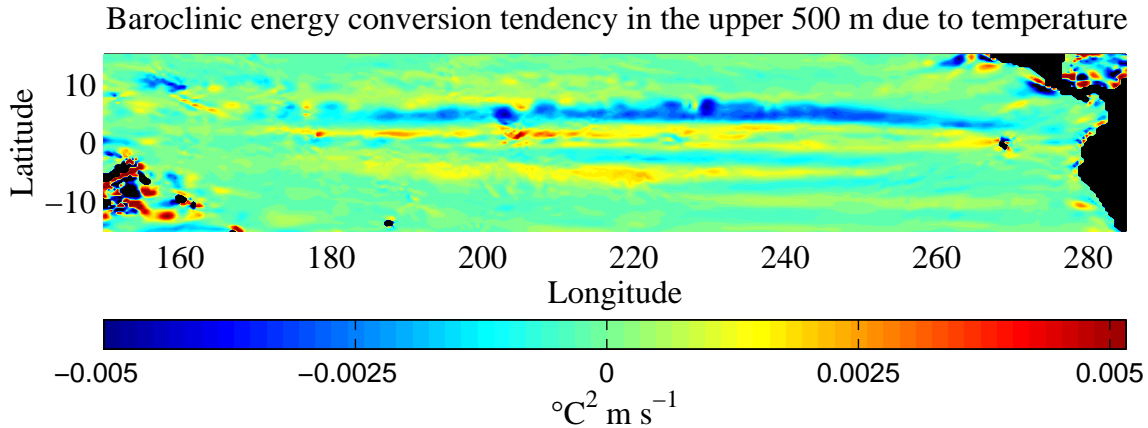
Figure 4.26: Eddy potential energy conversion tendency due to temperature, estimated by the depth integral of \overline{\mathbf{v}'\theta'} \cdot \nabla\overline{\theta} over the upper 500 meters. Negative values correspond to a conversion of mean flow energy to eddy potential energy, and positive values indicate a conversion of eddy potential energy to the mean flow energy.
