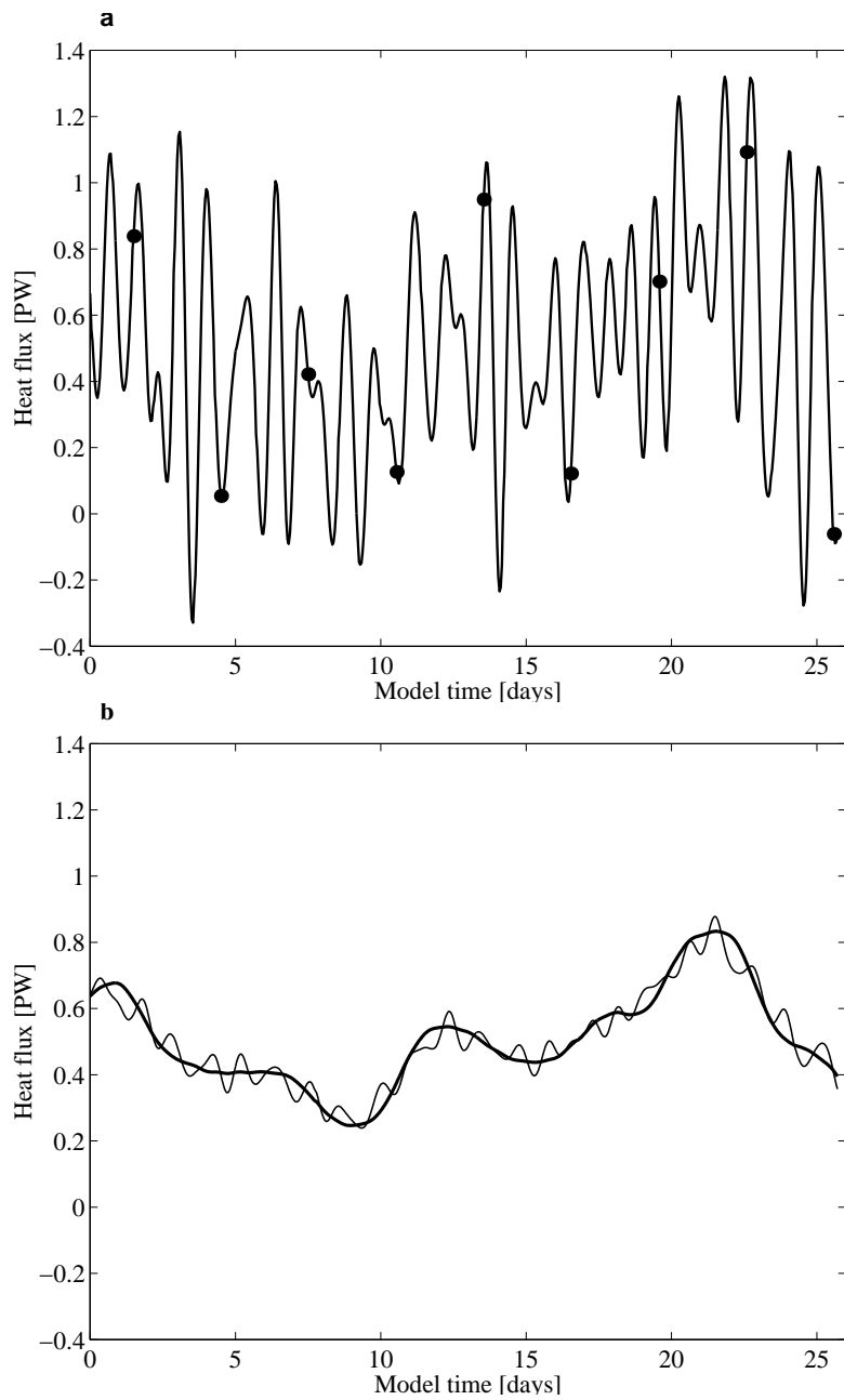
Figure 2.6: (a) Unfiltered heat transport time series at 25^{\circ}\text{N} in the Atlantic with the dots representing arbitrary once-per-3-days sampling. (b) Same results but using a 3-day running boxcar filter (thin solid line) and a 3 day running Hamming filter (heavy solid line) on the heat transport data.
