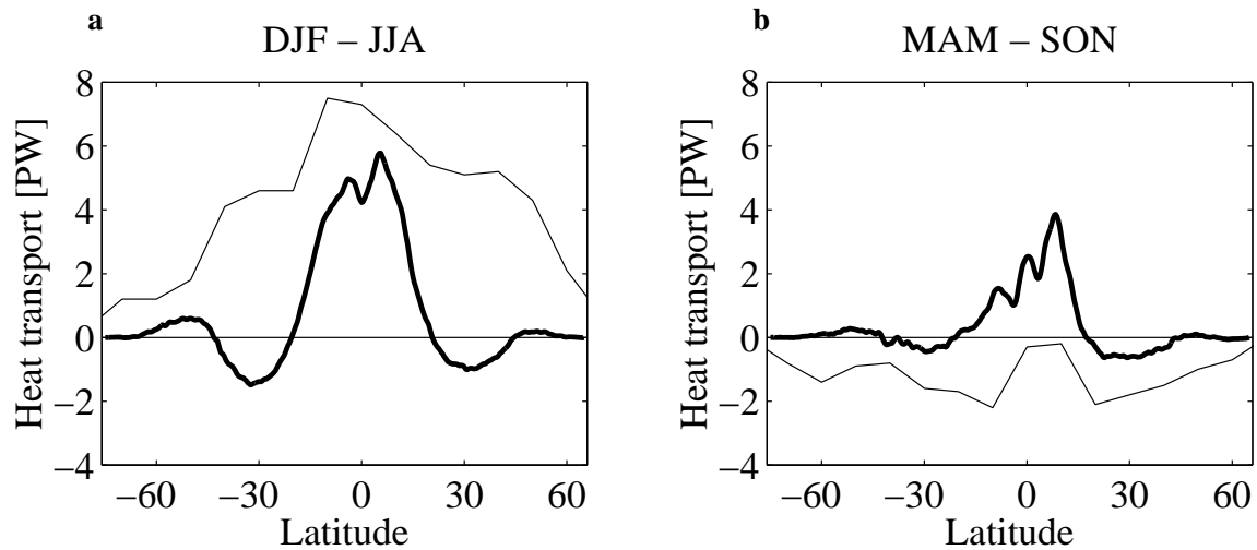
Figure 4.4: Annual cycle of ocean heat transport for the World Ocean from POCM (heavy line) and estimate of Carissimo et al. (thin line) for (a) average of December, January and February (DJF) minus June, July and August (JJA) and (b) average of March, April and May (MAM) minus September, October and November (SON).
