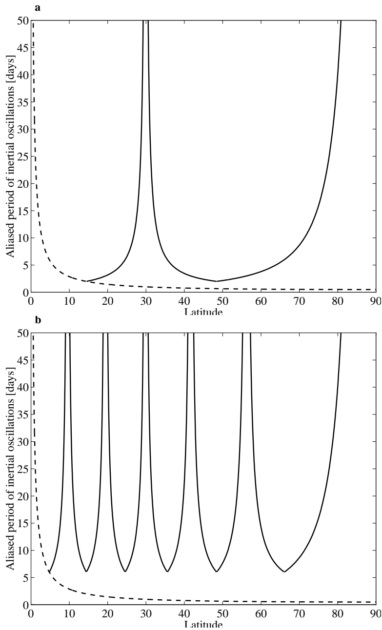
Figure 2.3: The true period of inertial oscillations (dashed) and their aliased period (solid) as a function latitude for sampling at (a) once per day and (b) once per 3 days.
