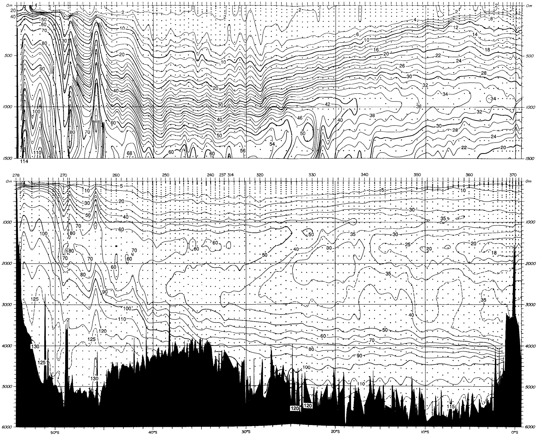
Figure 6. Vertical section of silica ( \mu\text{mol kg}^{-1} ) from Hydros 3/4, February–April 1989, based on discrete bottle data.
