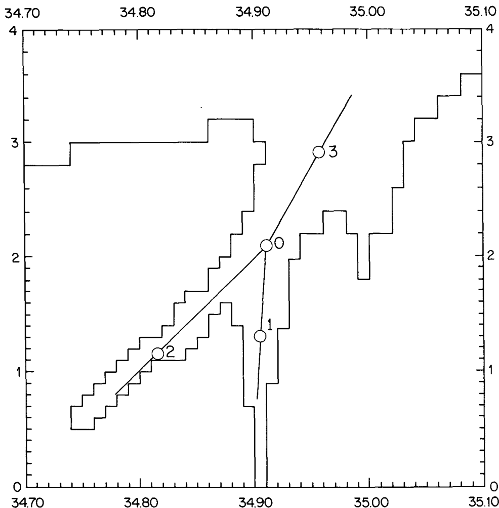
FIG. 2. Schematic configuration of the ridge lines showing their common intersection at point 0. The points 1, 2, and 3 are representative points chosen on the ridges for the purpose of determining the slopes of the lines, as in Table 1 (method A).
