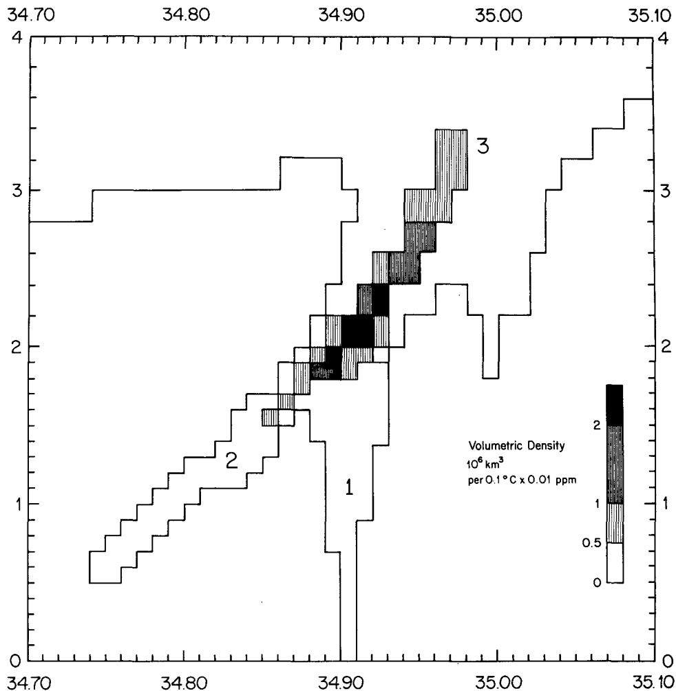
FIG. 1. Simplified version of the bivariate volumetric census of potential temperature and salinity for the North Atlantic Ocean from Wright and Worthington (1970). The ridges 1 and 2 represent bottom water from the Denmark Straits and Antarctic. The high ridge 3 is the large volume of North Atlantic Deep Water.
