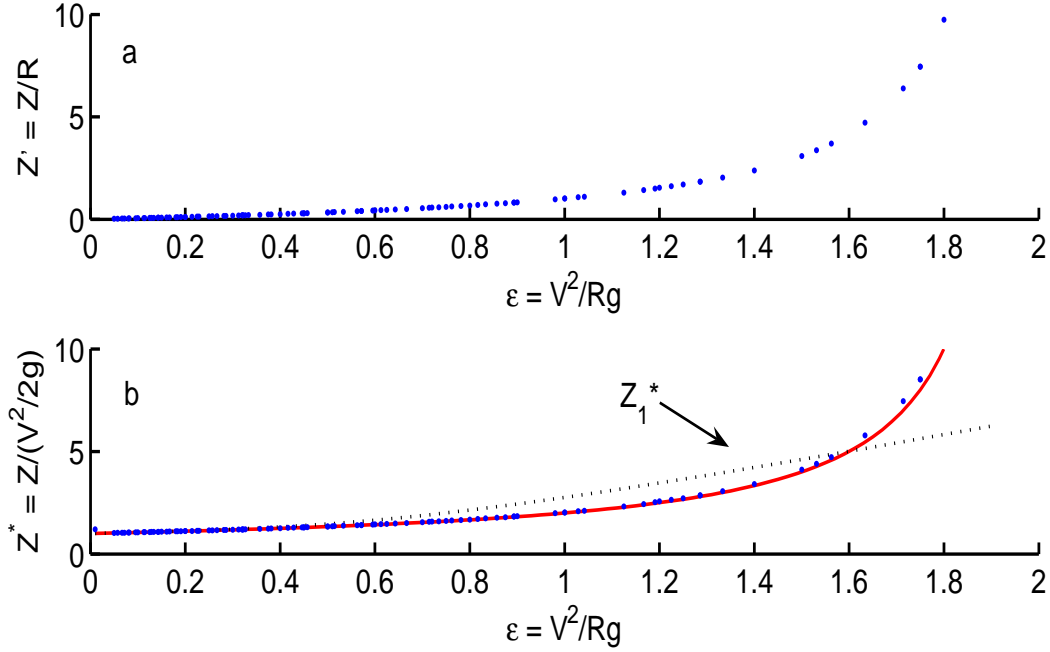
Figure 9: The maximum height of a projectile launched upwards at various speeds V from planets with various R and g . Each dot is the maximum height diagnosed from a numerical solution. In (a), the maximum height has been nondimensionalized by R , consistent with the initial basis set of nondimensional variables, Eq. (79). In (b), the basis set is one deduced from a scaling analysis (Section 7.3). Both of these indicate a clear-cut dependence of maximum height upon the single nondimensional parameter \epsilon = V^2/gR . Notice that as \epsilon approaches 2 the nondimensional height goes to infinity, indicating that the projectile has escaped the tug of gravity. The dotted line in (b) is the maximum height of the first order solution, Z_1^* , and the solid line that runs nearly through the data points is an approximate solution in which the effective gravitational acceleration is taken to be g(1 - \epsilon/2) ; both of these approximate solutions are developed in Section 7.4.
