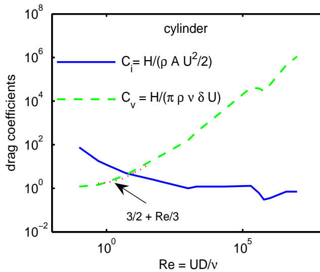
Figure 5: Drag coefficients of a sphere (a) and a cylinder (b) moving at a steady speed U through viscous fluid. Two forms of drag coefficient are shown here, the viscous drag coefficient is denoted by C_v (the dashed line), and the inertial drag coefficient denoted by C_i (the solid line, usually denoted C_d , and by far the most commonly encountered form). Note that C_v is O(1) (numerically and that it is approximately independent of Re ) if Re is very small, and that C_i is O(1) if the Reynolds number is very large. The inertial drag coefficients were read from Munson et al., Fig. 7.7 and Rouse, Figs. 125-126. 3,16
