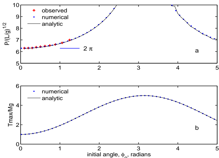
Figure 3: (a) The period of a simple pendulum as diagnosed from a series of numerical solutions (dots), as computed from theory that yields an elliptic integral that is also evaluated numerically (solid line), and as observed (crosses). The observations were acquired by measuring the time required for ten oscillations of a nearly conservative pendulum using an electronic stopwatch. The observed period is accurate to about 0.3%. The flexible line of this pendulum and the initial condition d\phi/dt = 0 limit the initial angle to about -\pi/2 < \phi_0 < \pi/2 . The period goes to infinity as \phi_0 \rightarrow \pi because the initial condition is \frac{d\phi}{dt}(t=0) = 0 . From dimensional analysis we expect that this F(\phi_0) holds for all simple, inviscid pendulums. (b) The maximum tension, T_{max} , diagnosed from a series of numerical solutions (dots) and as computed from energy conservation and the radial equation of motion (solid line); we had no way to measure this variable.
