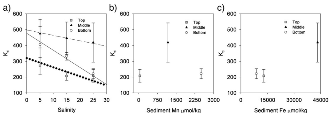
Fig. 7. Experimental distribution coefficients ( K_d ) plotted against a) salinity, b) sediment Mn (hydr)oxides and c) Fe (hydr)oxides. Data is the average of six time points during the 48 hour desorption experiment, and b) and c) contain data only from salinity 25. The linear fits between K_d and salinity in a) are represented by the dotted line (top, r^2=0.28 ), dashed line (middle, r^2=0.05 ) and solid line (bottom, r^2=0.57 ). Error bars represent the standard deviation of six K_d values.
