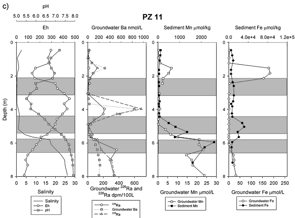
Fig. 2. Groundwater profiles of salinity, Eh, pH, ^{226}\text{Ra} , ^{228}\text{Ra} , Ba, Mn and Fe and sediment Mn and Fe for a) PZ 7, b) PZ 6 and c) PZ 11. Shaded regions in (c) indicate the depth range from which sediments for the adsorption/desorption experiments were collected.
