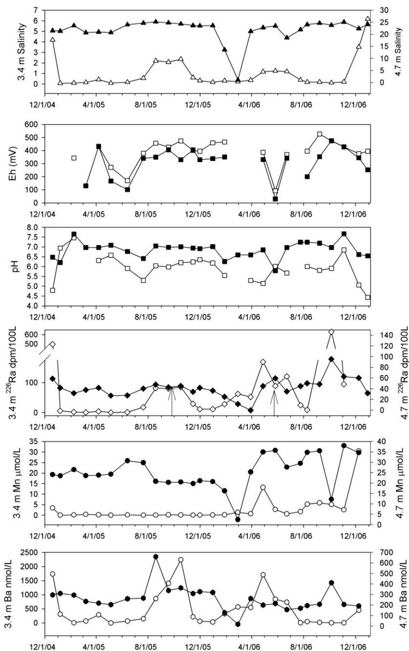
Fig. 6. Time series measurements at 3.4 m (open symbols) and 4.7 m (filled symbols) within the Waquoit Bay STE of salinity, Eh, pH, ^{226}\text{Ra} , dissolved Mn and dissolved Ba. Note the different scales for the parameters between the two depths.
