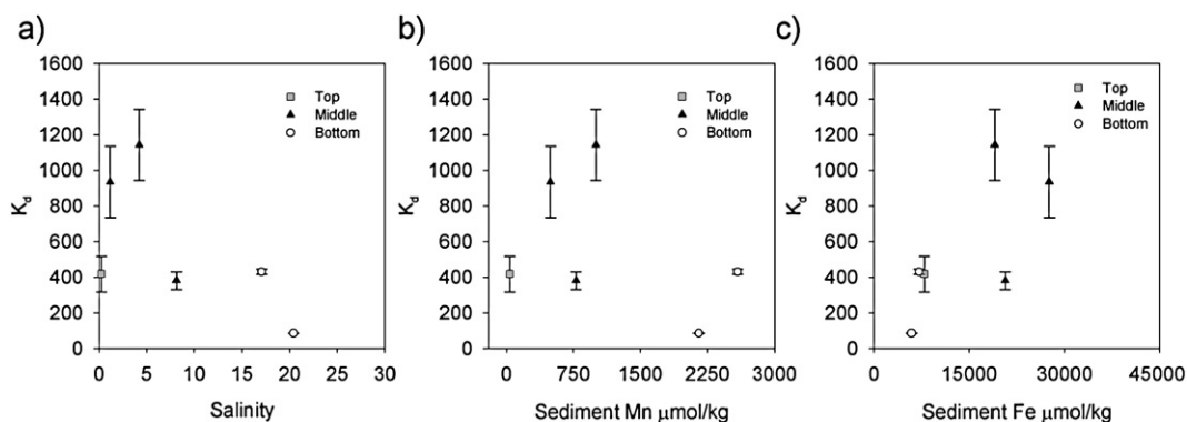
Fig. 8. In situ ^{226}\text{Ra} K_d s plotted against a) salinity, b) sediment Mn (hydr)oxides and c) Fe (hydr)oxides. Error bars represent analytical uncertainties.
