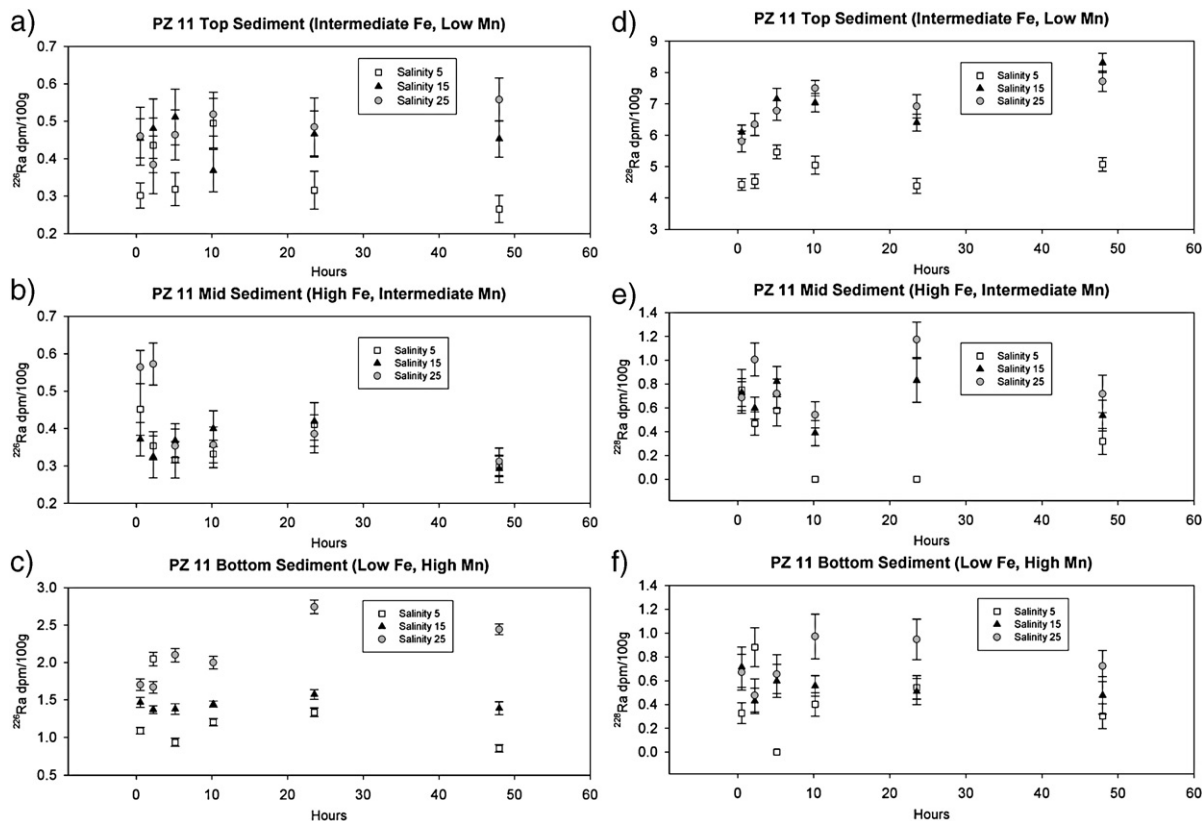
Fig. 3. Desorbed ^{226}\text{Ra} from PZ 11 (a) top, (b) middle, and (c) bottom and ^{228}\text{Ra} from PZ 11 (d) top, (e) middle, and (f) bottom at salinity 5 (empty squares), 15 (black triangles) and 25 (grey circles). Error bars represent analytical uncertainties.
