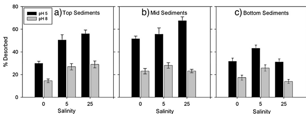
Fig. 4. Desorption from a) top, b) middle and c) bottom sediments at pH 5 (black) and 8 (grey) for salinity 0, 5 and 25. Note these sediments were spiked with ^{226}\text{Ra} prior to desorption (see methods section for details). Error bars represent analytical uncertainties.
