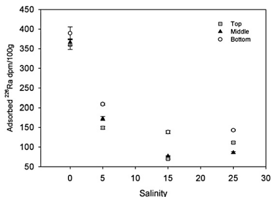
Fig. 5. ^{226}\text{Ra} adsorption capacity of PZ 11 sediments from the top, middle, and bottom versus salinity. Error bars are plotted for all data but are smaller than the symbol in some cases.
