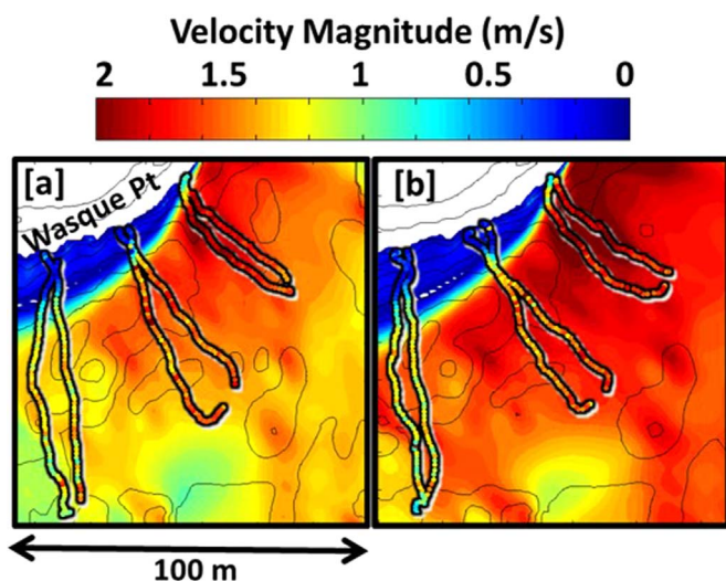
Fig. 2. Observed (colored symbols within black outlines of the boat transects) and simulated (color contours, scale above) currents near Wasque Point during approximately (a) mid- and (b) maximum-ebb tide. If model and data agree, the colors along the transect lines match the colors of the surrounding simulation contours. The observations (13 Jul 2015) from the ADCP transects are averaged over depth and over ~10 m along the track (boat speed ~1 m/s). The simulated currents are from 1-h model runs initialized with wave and tidal conditions corresponding approximately to those observed during the middle of each ~2-h long suite of transects. (For interpretation of the references to color in this figure legend, the reader is referred to the web version of this article.)
