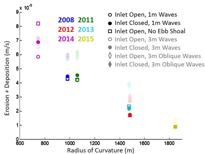
Fig. 4. The sum of the absolute values of simulated erosion and deposition along 400 m of the shoreline between 0- and 2-m water depths (Fig. 3c) versus the radius of curvature of the southeastern corner of Chappaquiddick Island in each of 6 years (colors, legend in upper right). Simulations used the bathymetry observed each year with the inlet open (open symbols), with the inlet artificially closed (closed symbols), with normally (circles) and obliquely (30° west of normal, diamonds) incident offshore wave directions, and with the ebb shoal removed artificially (open squares) for incident significant wave heights of 1 (dark colors) and 3 m (light colors). Inlet-open cases are not shown for 2015 because the inlet was closed. (For interpretation of the references to color in this figure legend, the reader is referred to the web version of this article.)
