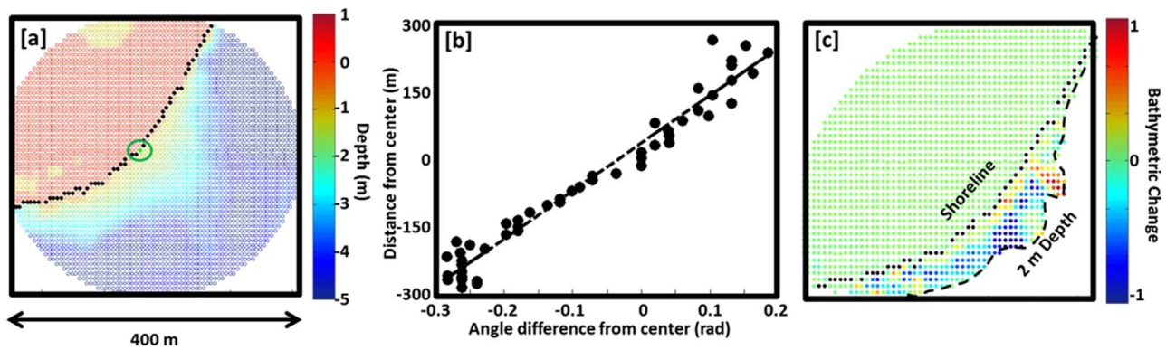
Fig. 3. (a) Color contours of elevation (relative to mean sea level, scale on right) on the southeast corner of Chappaquiddick Island near Wasque Point in 2011. The black dots are the shoreline, and the green circle is the center of the radius of curvature. (b) Distance from the center point versus angle of tangents to the shoreline (relative to a tangent at the center). The slope of the least squares fit (dashed line) is the radius of curvature. (c) Color contours of erosion (blue) and deposition (red) (scale on right, arbitrary units) within a region between the shoreline (black dotted curve) and 2 m depth (black dashed curve). (For interpretation of the references to color in this figure legend, the reader is referred to the web version of this article.)
