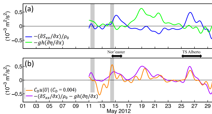
Figure 9. Subtidal, demeaned shoals (a) wave forcing -(\partial S_{xx}/\partial x)/\rho_0 (blue curve) and pressure gradient -gh(\partial\eta/\partial x) (green curve) and (b) bottom stress (orange curve, C_D = 0.004 , from Figure 7f) and wave radiation-stress plus pressure gradients -(\partial S_{xx}/\partial x)/\rho_0 - gh(\partial\eta/\partial x) (purple curve) versus time. The two curves in Figure 9b are correlated ( r^2 \sim 0.45 ) at 95% confidence levels. Gray vertical stripes are times of cross-inlet transects (white line, Figure 1b) with the boat-mounted current profiler (see Appendices A and B). Times of a nor'easter and tropical storm Alberto are indicated with black arrows.
