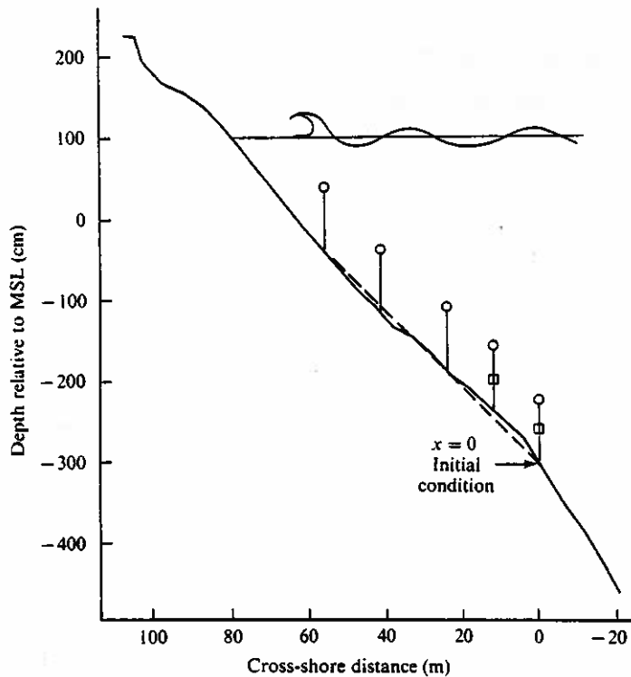
FIGURE 1. Measured beach profile, constant-slope approximation (dashed line), and instrument locations along a line perpendicular to the beach: ○, pressure gauges; □, bidirectional current meters.
