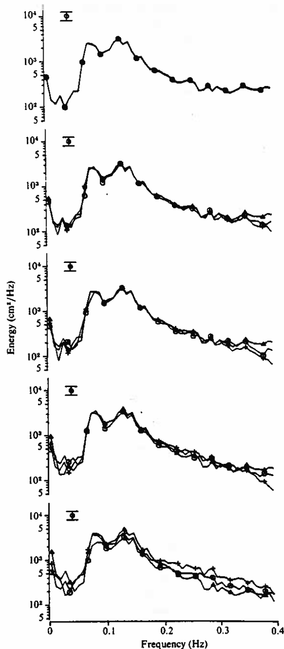
FIGURE 2. Energy spectra for the 30 January data. From top to bottom, x = 0 ( h = 4.1 m), 12 (3.5 m), 24 (2.9 m), 41 (2.0 m), and 56 m (1.2 m). \circ , data; \blacktriangle , directional LFDT; + , nonlinear model. There are 144 degrees of freedom (d.o.f.) and the bars indicate 95% confidence limits.
