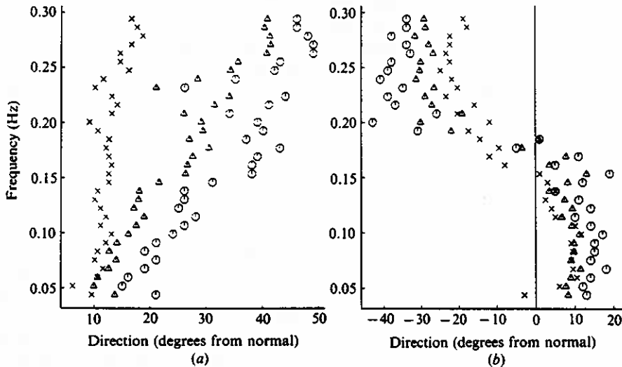
FIGURE 12. Direction, relative to the beach normal, of the peak of the directional spectra for each frequency band. ○, angle measured in 9 m depth; △, angle predicted by Snell's law in 3–4 m depth; ×, angle measured in 3–4 m depth. (a) 2 February; (b) 12 February.
