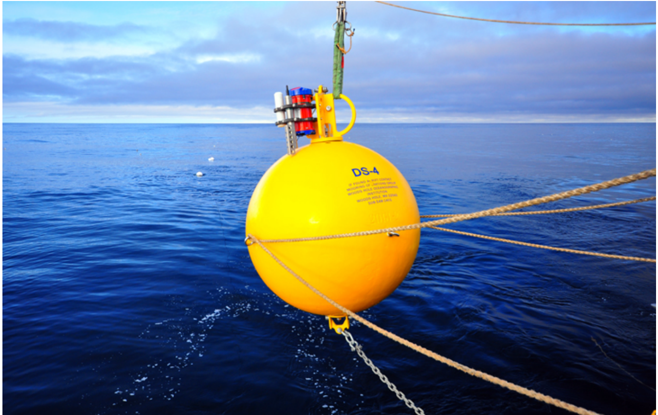
1. 60" Syntactic Sphere with attached current profiler - keeps the mooring line tight (Rachel Fletcher)
