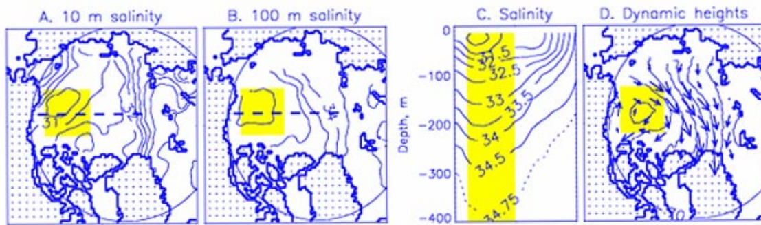
Fig. 1. Winter salinity at 10 (A) and 100 (B) meters. Section C shows the salinity distribution along the dashed line. Dynamic heights relative to 200 db and direction of geostrophic circulation are shown in D. There is a large-scale (1500x1500x0.4 cu. km) anticyclonically rotating lens of fresh water (BG circulation cell) in the Canadian Basin of the Arctic Ocean.
