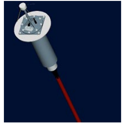
Figure 19. METOCEAN ice-beacon
