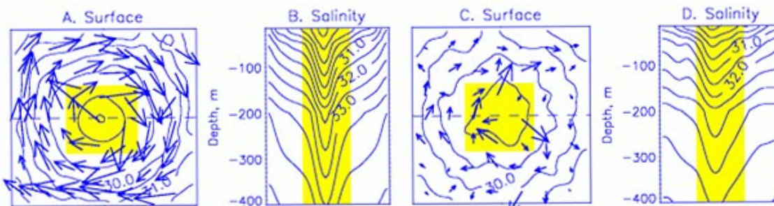
Fig. 3. Results of numerical experiments with a 3-D model in the 2000kmx2000kmx1.5km ideal basin. The basin is initially horizontally uniform but vertically stratified, then it was forced for 9 months by anticyclonic (A and B) and then 3 months by cyclonic (C and D) symmetric winds. (A) and (C) show surface salinity and currents. (B) and (D) show salinity sections along dashed line in (A) and (C). Anticyclonic winds generate downwelling in the central basin and upwelling along boundaries. Cyclonic winds lead to the upwelling in the central basin and downwelling along boundaries. Anticyclonic forcing (A) is similar to the winter Arctic conditions, and the salinity structure in (B) resembles Fig. 1C. Fig. 3C shows surface salinity and currents after 3 months of cyclonic wind forcing. Circulation pattern of this figure is similar to the ice drift pattern in Fig. 2D (summer ice drift). The circulation is still anticyclonic but is weaker than in winter. Salinity distribution in (D) could be observed in summer when the cyclonic wind forcing leads to the release of freshwater from deep layers to upper layers. Observations are needed in the Beaufort Gyre to test this hypothesis.
