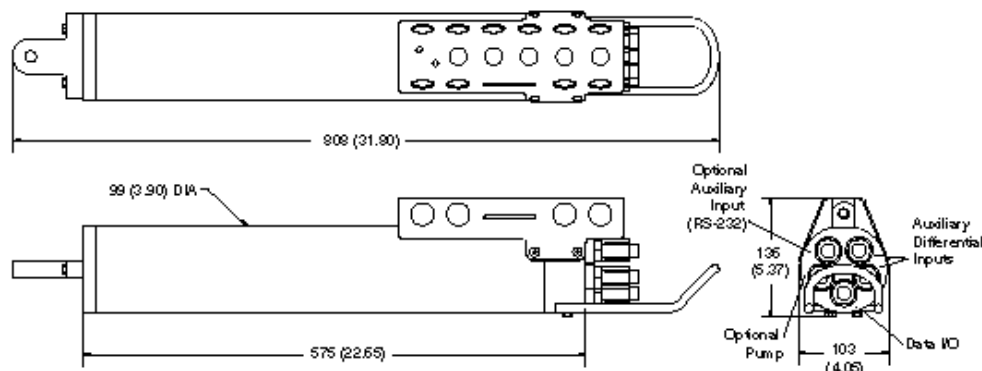
Figure 18. Bottom pressure recorder
