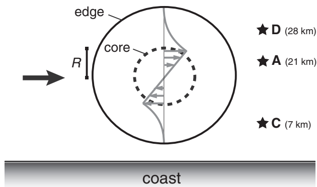
Fig. 6. Schematic of an anticyclonic, low-salinity eddy propagating by the mooring array (shown to approximate scale, with distances of each mooring given from the coast). The eddy has a core of radius R (dashed circle), a fresh anomaly out to its edge (solid circle), and is moving from left to right. Gray lines show the velocity structure of an ideal Rankine vortex.
