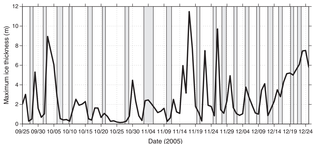
Fig. 4. Time-series of daily maximum ice draft (m) measured by the Upward Looking Sonar instrument on the center mooring during a three-month period of fall 2005. Shading indicates occurrences of low-salinity pulses observed by the mooring array.
