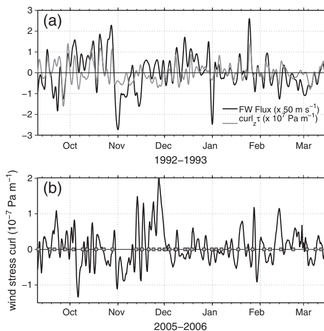
Fig. 9. (a) Time series of wind stress curl, \text{curl}_z\tau ( \times 10^{-7} \text{ Pa m}^{-1} ), averaged over Hudson Bay and the freshwater flux ( \times 50 \text{ m s}^{-1} ) calculated from the DFO mooring in 1992–1993. The freshwater flux estimate is lagged by 1.5 days to show the maximum correlation between the time series. (b) Wind stress curl, \text{curl}_z\tau ( \times 10^{-7} \text{ Pa m}^{-1} ), averaged over Hudson Bay calculated from the NCEP reanalysis data for 2005–2006. The timing of low-salinity events observed propagating by the mooring array are shown (gray squares) lagged by the product of their along-strait speed and the distance to the western entrance of Hudson Strait (~310 km).
