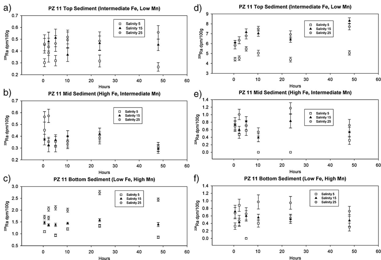
Fig. 3. Desorbed 226 Ra from PZ 11 (a) top, (b) middle, and (c) bottom and 228 Ra from PZ 11 (d) top, (e) middle, and (f) bottom at salinity 5 (empty squares), 15 (black triangles) and 25 (grey circles). Error bars represent analytical uncertainties.
