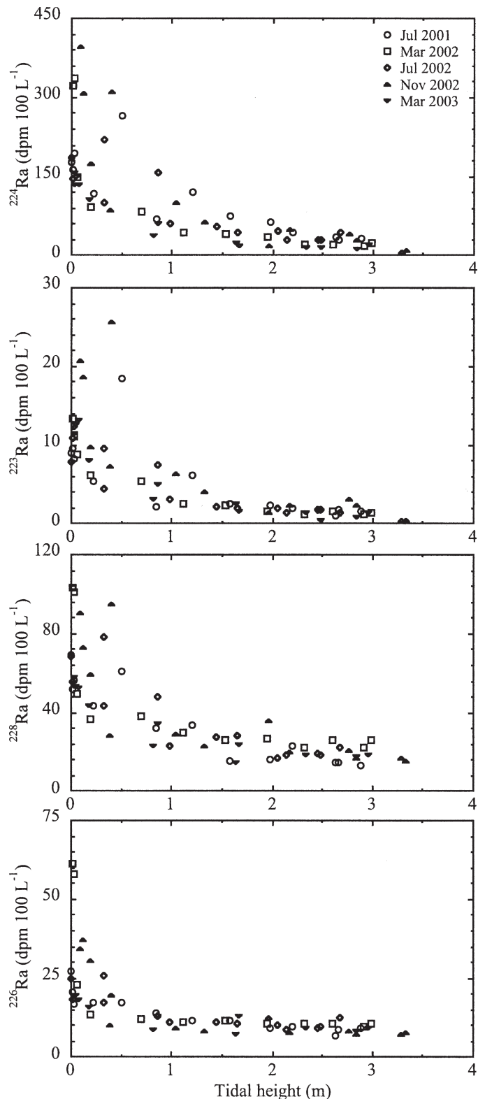
Fig. 2. Radium isotopes versus tidal height for the time-series surface-water samples.
