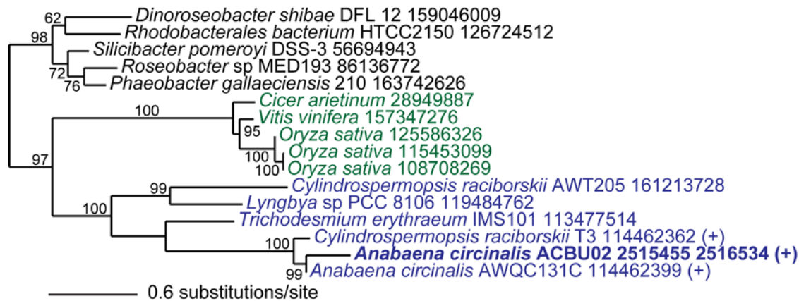
Figure 3. Phylogeny of sxtN . ML phylogenetic tree of sxtN (sulfotransferase) that represents saxitoxin-related genes of cyanobacterial origin that is potentially from members of the Oscillatoriales. ML bootstrap values (when \geq 50\% ) are indicated at the nodes. The branch lengths are proportional to the number of substitutions per site (see scale in the figure). Cyanobacterial taxa are shown in blue text, non-cyanobacterial prokaryotes in black text, and eukaryotes (Plantae) in green. The tree has been rooted on the branch leading to the non-cyanobacterial prokaryotes. doi:10.1371/journal.pone.0005758.g003
