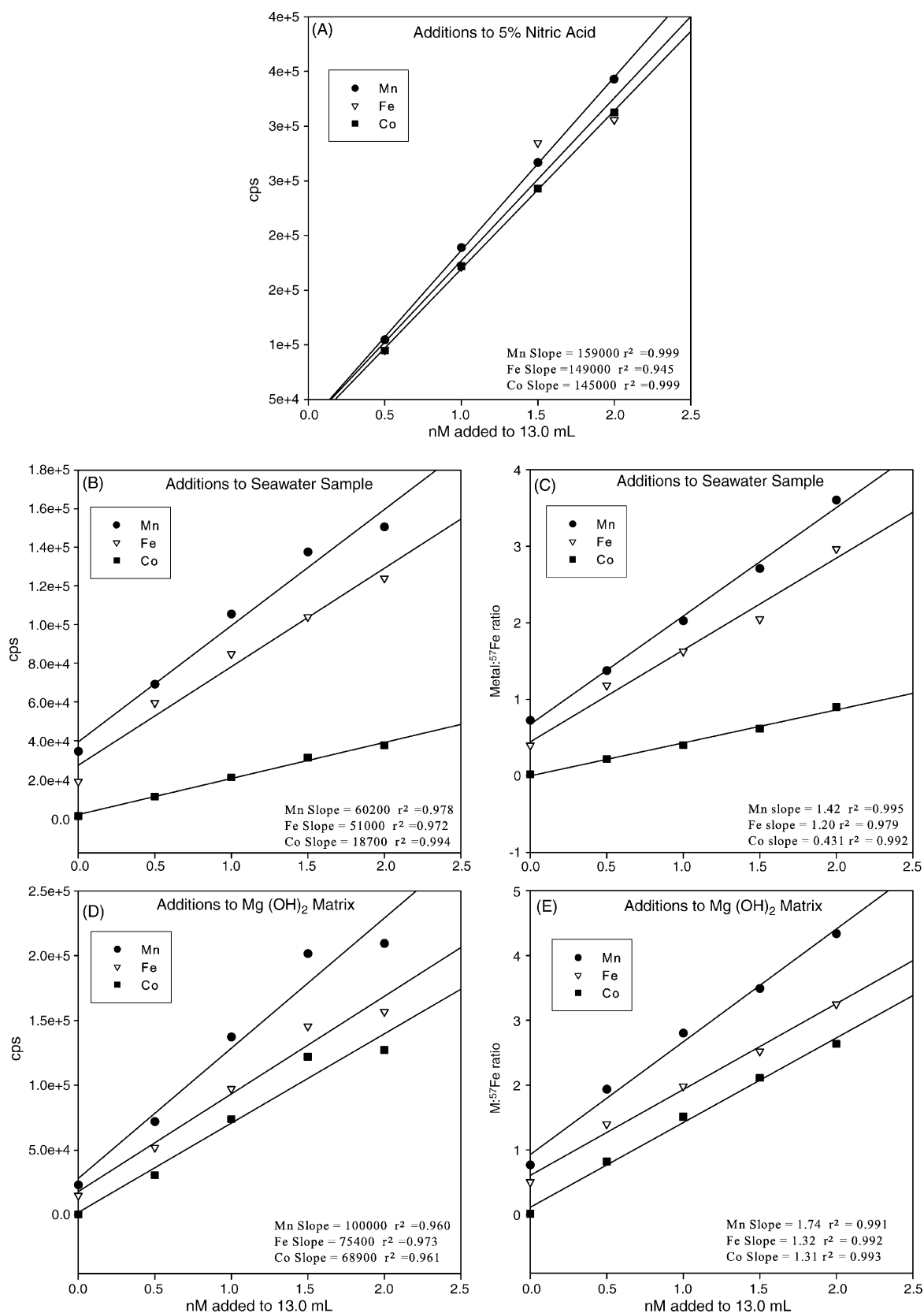
Fig. 4. Analysis of Mn, Fe, and Co additions to (A) 5% nitric acid, (B) seawater samples (additions prior to precipitation), (C) seawater samples (additions prior to precipitation) normalized to ^{57}\text{Fe} , (D) \text{Mg}(\text{OH})_2 matrix redissolved in 5% nitric acid (additions after precipitation), and (E) \text{Mg}(\text{OH})_2 matrix redissolved in 5% nitric acid (additions after precipitation) normalized to ^{57}\text{Fe} . While all three elements have similar ionization efficiencies (panel A), the scavenging efficiencies of Fe and Mn are significantly better than that of Co (panels B and C). Decreases in slope in panels B–E are caused by the \text{Mg}(\text{OH})_2 matrix effects as well as the poor scavenging efficiency of cobalt. When normalized to ^{57}\text{Fe} significantly higher r^2 values are obtained relative to the counts per second values.
