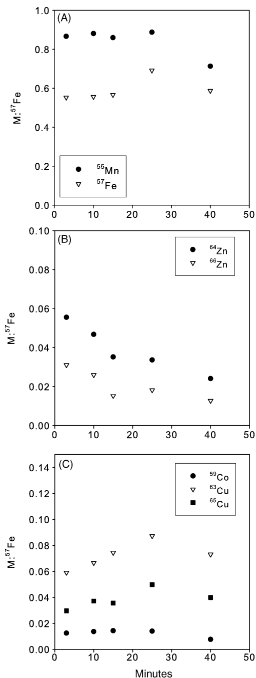
Fig. 5. The effect of precipitation time on the scavenging of (A) Mn, Fe, (B) Zn, (C) Co and Cu. Longer scavenging times do not appear to increase the scavenging of all elements with the exception of Cu. Fe, Mn, and Co scavenging remains relatively constant despite longer precipitation times. Zn appears to decrease relative to ^{57}\text{Fe} , and Cu appears to increase with longer durations.
