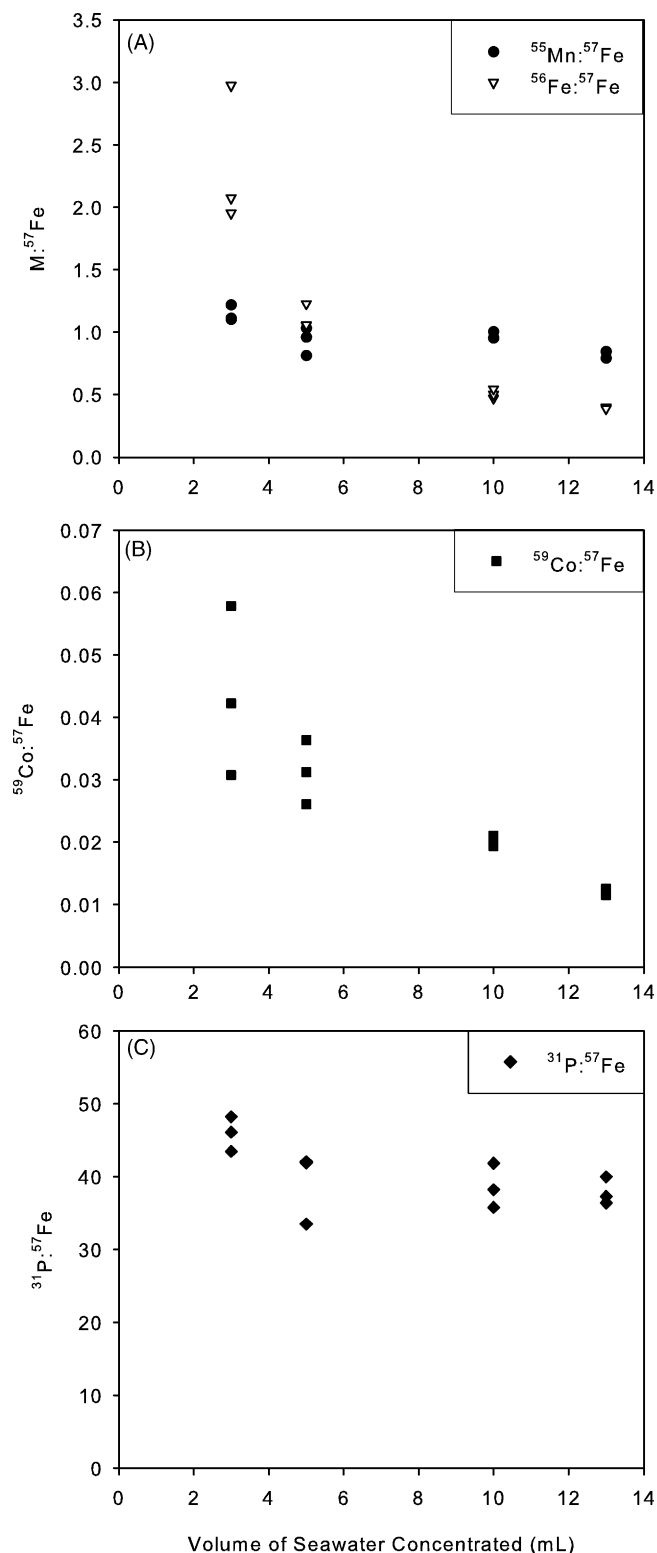
Fig. 1. The influence of the volume of seawater precipitated on the precision and signal-to-blank ratio. Previous studies have typically used 1.3 mL volumes. Increases in precipitated volume greatly increase precision and asymptotically approach a “correct” ratio once the signal is sufficiently higher than the blank. The precision at the 3 and 5 mL volumes are somewhat exaggerated due to the need to dilute the samples by an additional 1.7-fold to reduce Mg interferences (see text). Blank corrections were purposely omitted to demonstrate the influence of sample volume on the blank.
