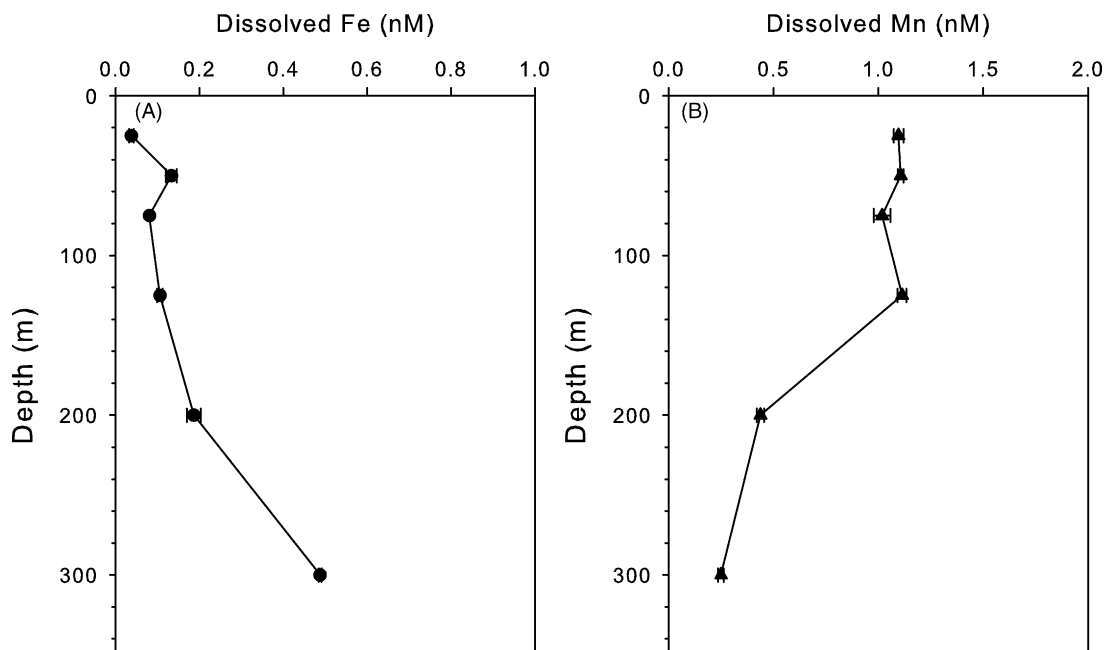
Fig. 9. Vertical profiles of (A) iron and (B) manganese in the Central Pacific south of the Hawaiian Islands ( 12^\circ 42.35'\text{N} , 158^\circ \text{W} , Station 7, KM0405) measured using the protocol described in this study.
