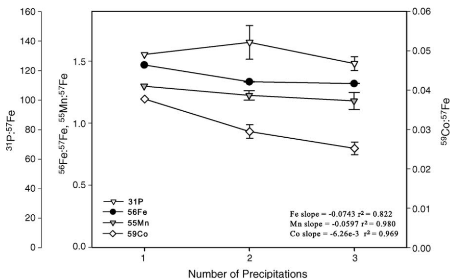
Fig. 3. Precipitation of previously precipitated seawater to examine recovery, using ^{57}\text{Fe} spiked aliquots for successive precipitations (aliquots are 5% of original volume).
