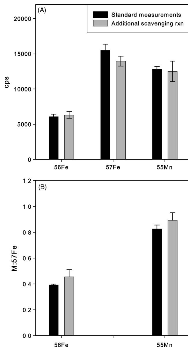
Fig. 7. \text{Mg}(\text{OH})_2 precipitates were exposed to fresh seawater sample (without added ^{57}\text{Fe} ) to examine if the precipitate when resuspended could scavenge additional Fe or Mn. (A) Fe and Mn presented in counts per second show no significant change when exposed to fresh seawater. (B) Ratios relative to ^{57}\text{Fe} are presented, correcting for losses of \text{Mg}(\text{OH})_2 . Error bars reflect standard deviation of triplicate analyses. These data suggest that the initial precipitation reaction, rather than the exposure to the already formed \text{Mg}(\text{OH})_2 , is when the metal preconcentration occurs.
