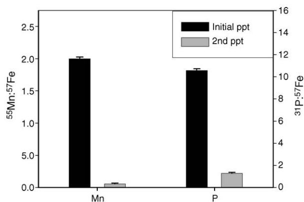
Fig. 6. The seawater supernatant from precipitated samples was decanted and reprecipitated to examine if further Mn or P could be recovered. Solid bars indicate the ^{55}\text{Mn}:^{57}\text{Fe} and ^{31}\text{P}:^{57}\text{Fe} ratio of the initial sample, and grey bars indicate those ratios on 7 mL of the supernatant. Error bars reflect standard deviation of triplicate analyses. Negligible Mn is concentrated from the supernatant, and a small portion of P is concentrated.
