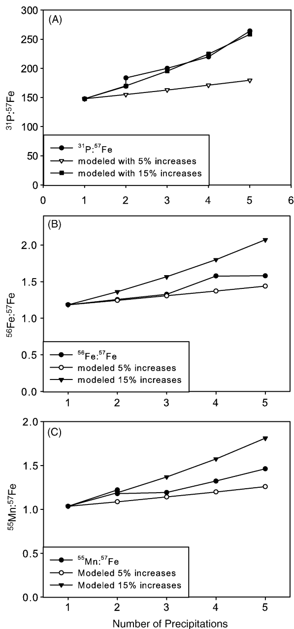
Fig. 2. Precipitation of previously precipitated seawater to examine recovery, without the use of ^{57}Fe spiked aliquots for successive precipitations (aliquots are 5% of original volume).
