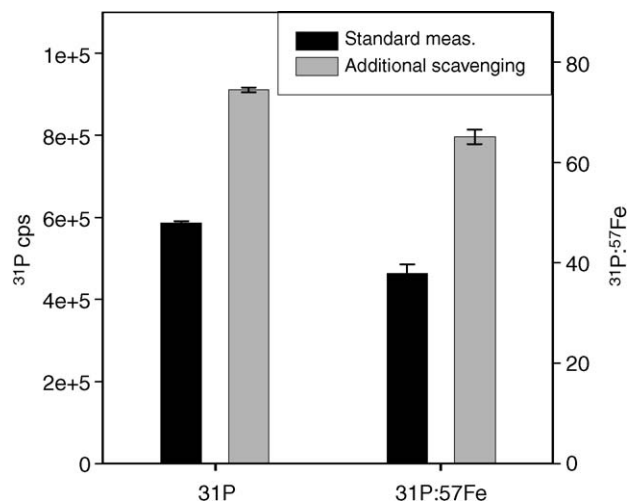
Fig. 8. \text{Mg}(\text{OH})_2 precipitates were exposed to fresh seawater sample (without added ^{57}\text{Fe} ) to examine if the precipitate when resuspended could scavenge additional P. ^{31}\text{P} presented in counts per second increases significantly when exposed to fresh seawater. Ratios relative to ^{57}\text{Fe} are presented, correcting for losses of \text{Mg}(\text{OH})_2 . These data indicate that unlike for Fe and Mn (see Fig. 7), the \text{Mg}(\text{OH})_2 precipitate is capable of scavenging P from seawater. Error bars reflect standard deviation of triplicate analyses.
