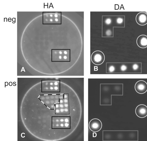
Fig. 4. In situ detection of Pseudo-nitzschia spp. and domoic acid (DA) in Monterey Bay March 2006 using the ESP. A) DNA array with probes for Pseudo-nitzschia australis , P. multiseriis/pseudodelicatissima , Alexandrium catenella , and Heterosigma akashiwo (HA array). Only control spots are outlined as targeted species are below detection level. B) Protein array for DA, corresponds to (A). Circled spots are IgG controls confirming consistency of detection chemistry. Spots in red rectangles are DA conjugate. Maximum intensity in DA conjugate spots indicates DA levels are below detection limit, whereas decreasing spot intensity indicates presence of DA (competitive ELISA). C) HAB array from a later time indicates the presence of P. australis (spots bounded by dashed lines) and P. multiseriis/pseudodelicatissima (spots bounded by dotted lines), both of which can produce DA. D) DA array that corresponds to (C); circled spots are IgG controls; spots in rectangles are DA conjugate; the DA conjugate spots are considerably dimmed, indicating the presence of this toxin (from Doucette et al. and Greenfield et al. , in prep.).
