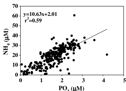
Fig. 12. \text{NH}_4^- versus \text{PO}_4^{3-} at VM5 for the surface concentrations from the time series from 1986 to 2001. The regression equation of \text{NH}_4^- to \text{PO}_4^{3-} and the correlation coefficients r are given (data from EPD, Hong Kong).
