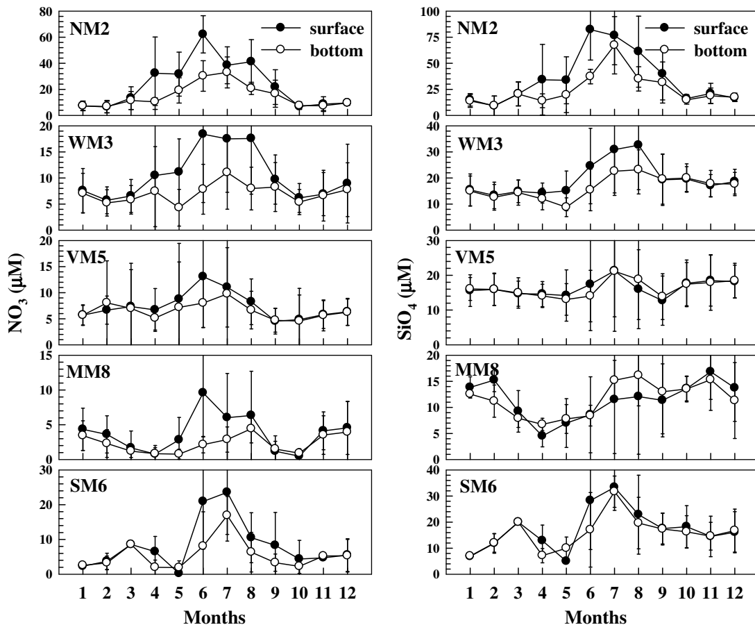
Fig. 3. Monthly average \text{NO}_3 and \text{SiO}_4 at the surface and bottom at five stations from 1986 to 2001. Vertical bars indicate \pm 1 SD. Note the different concentration scale for different stations (data from EPD, Hong Kong).
