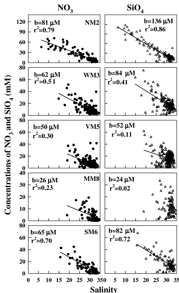
Fig. 10. Concentrations of \text{NO}_3 and \text{SiO}_4 versus salinity for the surface data for five stations from the time series from 1986 to 2001. The graphs with lines indicate a significant correlation between the two variables and the correlation coefficients are represented by r . The intercept of the regression line is represented by b (data from EPD, Hong Kong).
