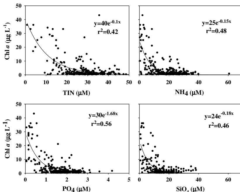
Fig. 13. Chl a concentration versus nutrients (TIN, NH 4 , PO 4 and SiO 4 ) at VM5 for the surface data from the time series from 1986 to 2001 (data from EPD, Hong Kong). The regression equation of NH 4 to PO 4 and the correlation coefficients r are given.
