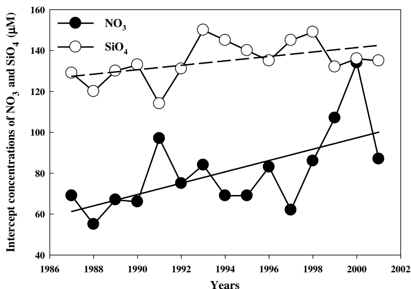
Fig. 11. Intercept concentrations of \text{NO}_3^- and \text{SiO}_4^{2-} at surface at NM2 from 1986 to 2001. p_{\text{NO}_3} < 0.05 and p_{\text{SiO}_4} > 0.05 , indicates that the correlation is significant for \text{NO}_3^- , not \text{SiO}_4^{2-} at the 0.05 level (2-tailed test) (data from EPD, Hong Kong).
