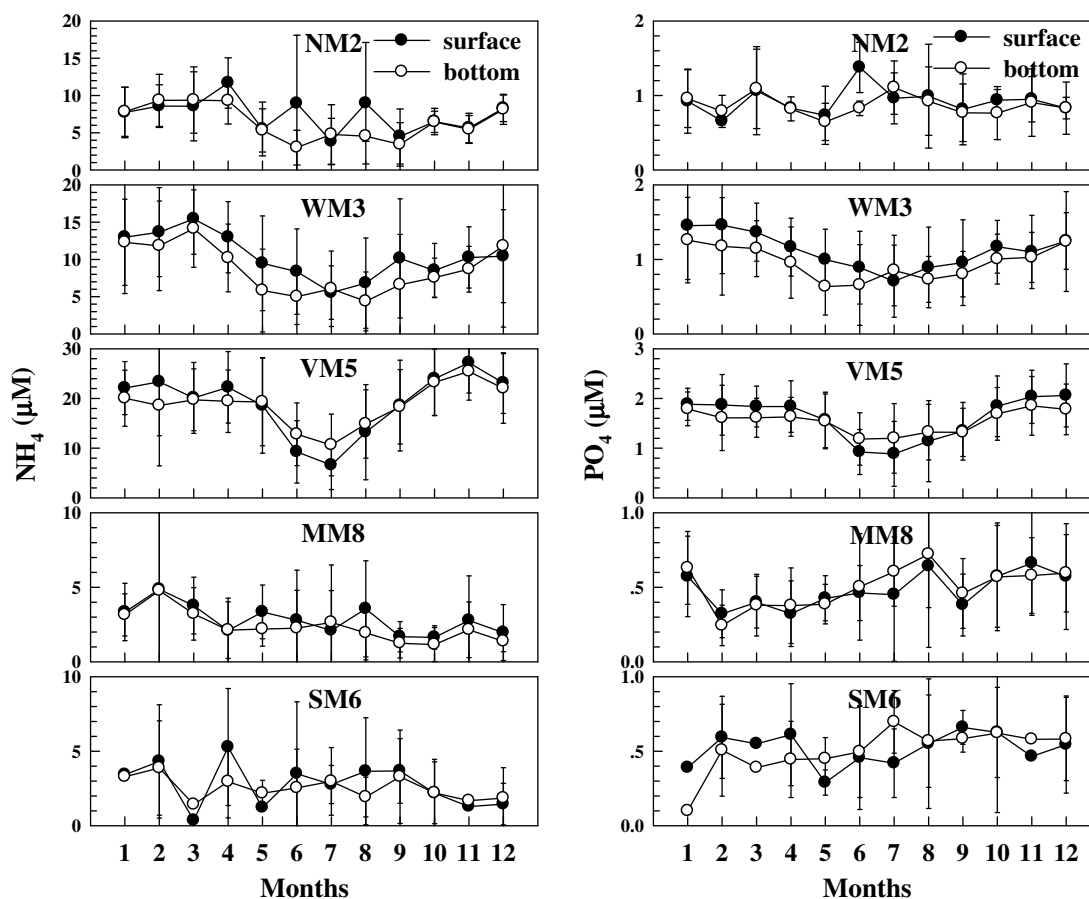
Fig. 4. Monthly average \text{NH}_4 and \text{PO}_4 at the surface and bottom at five stations from 1986 to 2001. Vertical bars indicate \pm 1 SD. Note the different concentration scale for different stations (data from EPD, Hong Kong).
