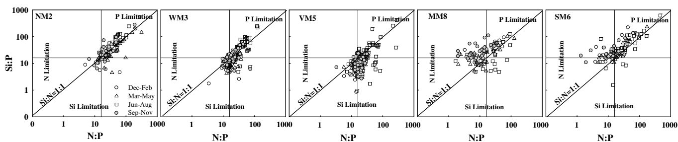
Fig. 8. Scatter diagrams of atomic nutrient ratios for the surface water during spring ( \Delta , March–May), summer ( \square , June–August), autumn ( \bullet , September–November) and winter ( \circ , December–February); N, P and Si represent dissolved inorganic N, P, and Si. Stoichiometric (=potential) limitation for N, P, and Si is indicated by the number of data points in the various quadrants (data from EPD, Hong Kong).
