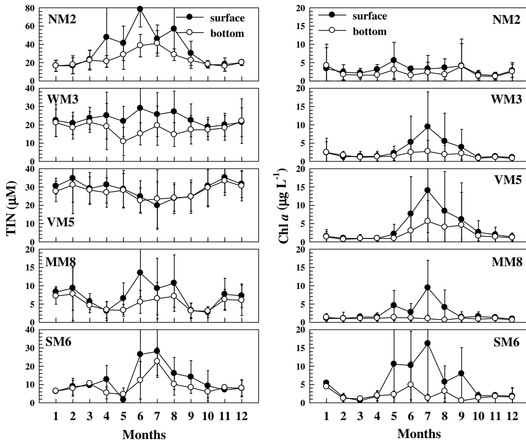
Fig. 5. Monthly average TIN ( =\text{NO}_3 + \text{NH}_4 + \text{NO}_2 ) at the surface and bottom at five stations from 1986 to 2001. Vertical bars indicate \pm 1 SD. Note the different concentration scale for different stations (data from EPD, Hong Kong).
