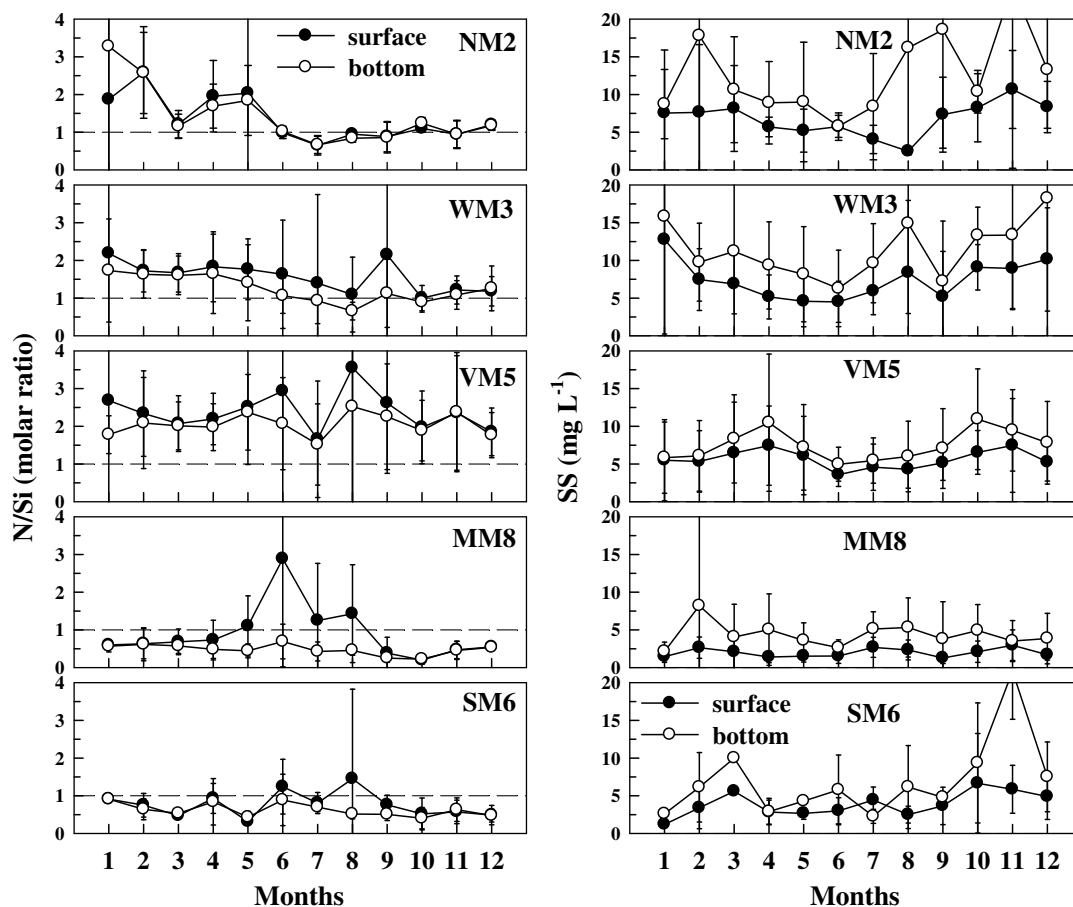
Fig. 7. Monthly average N:Si ratios and suspended solids (SS) at the surface and bottom at five stations from 1986 to 2001. Vertical bars indicate \pm 1 SD. The horizontal dashed line indicates a Redfield N:Si ratio of 1:1 (data from EPD, Hong Kong).
