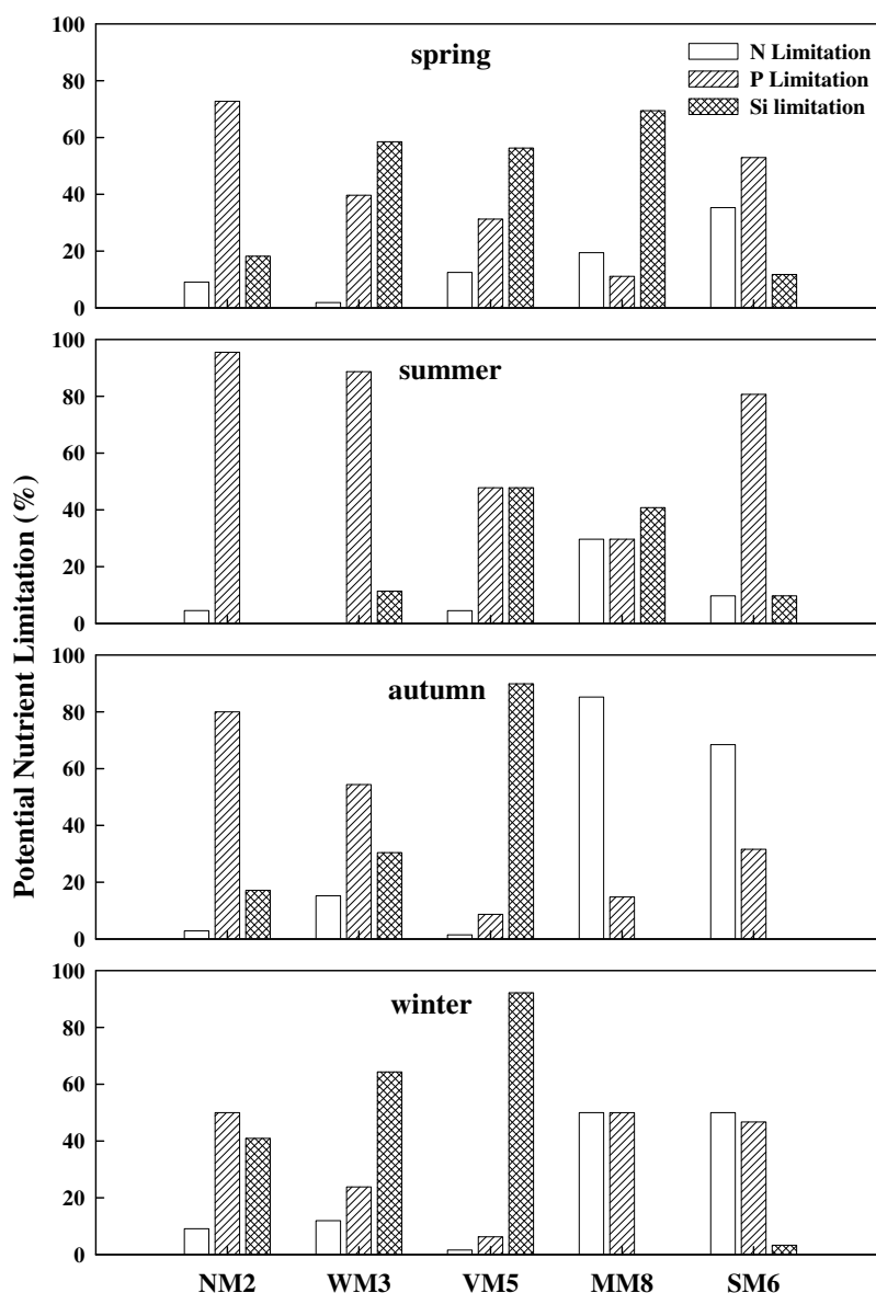
Fig. 9. Potential (%) N, P or Si limitation determined from plots in Fig. 8 for surface waters during spring (March–May), summer (June–August), autumn (September–November) and winter (December–February) at five stations in Hong Kong Waters from 1986 to 2001 (data from EPD, Hong Kong).
