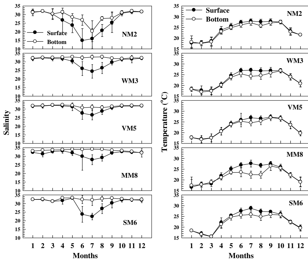
Fig. 2. Monthly average salinity and temperature at the surface and bottom at five stations from 1986 to 2001. Vertical bars indicate \pm 1 SD (data from EPD, Hong Kong).
