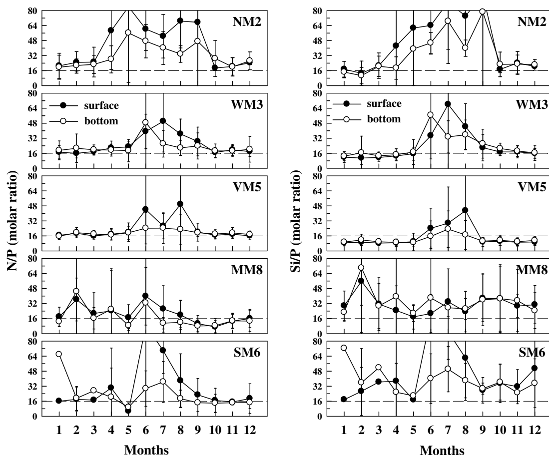
Fig. 6. Monthly average N:P and Si:P ratios at the surface and bottom at five stations from 1986 to 2001. Vertical bars indicate \pm 1 SD. The horizontal dashed line indicates the Redfield ratios of 16:1 for N:P and Si:P (data from EPD, Hong Kong).
