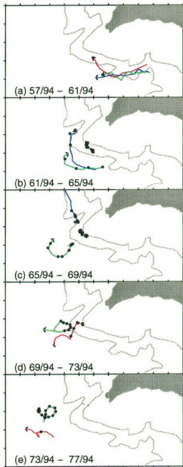
FIG. 11. Time sequence of four-day track segments for the three floats deployed on K23, showing meddy formation near Cape St. Vincent. Floats shown are am115 (K2305A, red), am139 (K2307, blue), and am129 (K2307A, green). Am129 ended up in the core of meddy whereas the other two did not. Area shown is the same as in Fig. 9. Sequence starts on yearday 57/94 and continues for 20 days. Dots along the tracks indicate where the floats observed T \geq 12.0^\circ\text{C} . The 1000-m and 2000-m isobaths are indicated by gray lines.
