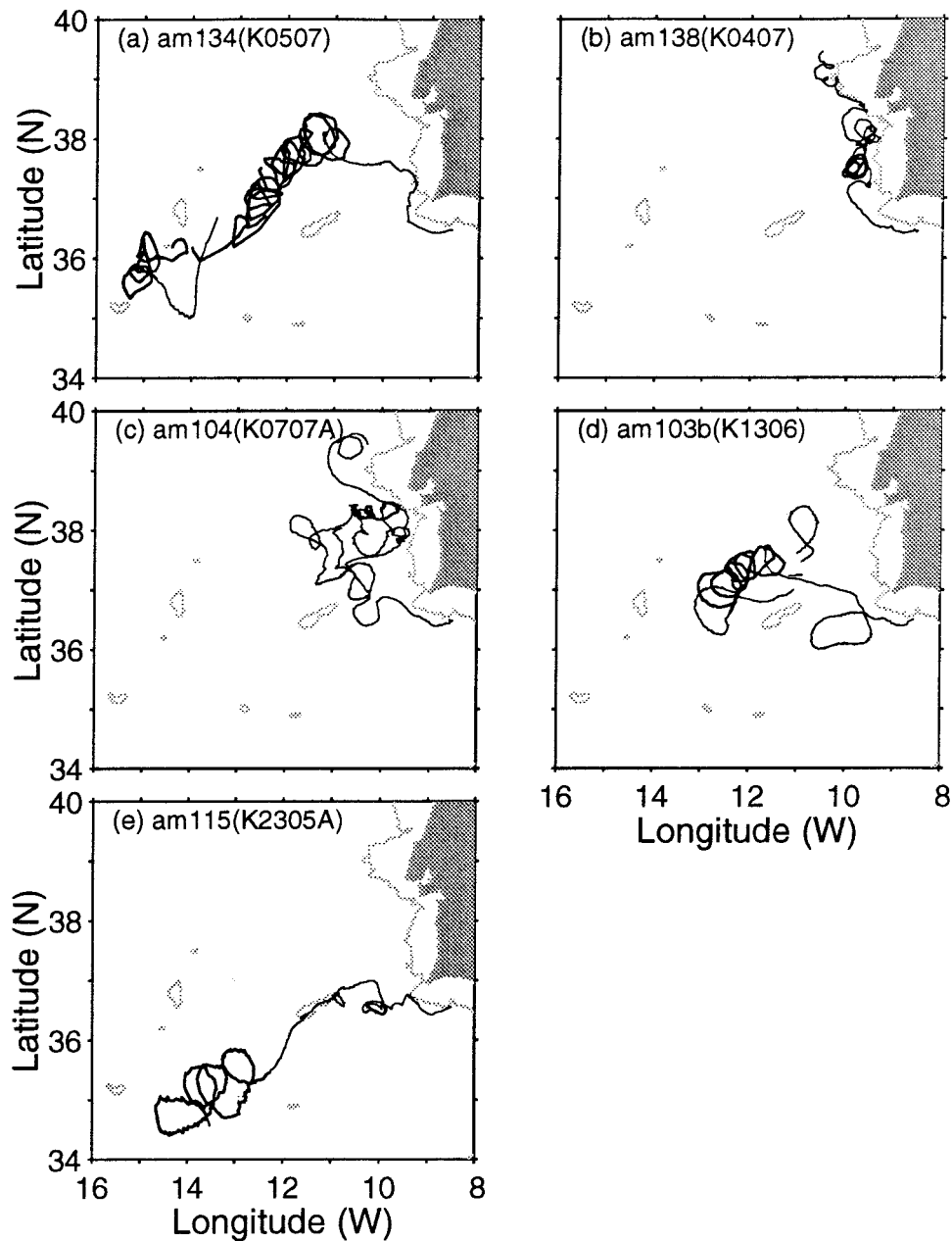
FIG. 20. Trajectories of five floats entrained into meddies during AMUSE: (a) am134 (K0507); (b) am138 (K0407); (c) am104 (K0707A); (d) am103b (K1306); and (e) am115 (K2305A). See Table 2 for statistical information.
