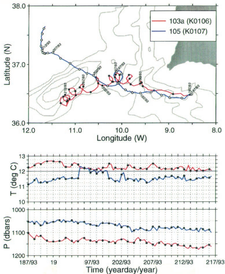
FIG. 6. Event 1: Trajectories of am103a (K0106, red) and am105 (K0107, blue) launched on 5 July 1993, yearday 186/93. All 8-h float positions are connected by line segments, and 24-h positions are indicated by circles along the track. Filled circles indicate where T > 12.0^{\circ}\text{C} . Positions are labeled at regular intervals with the date in yearday/year. Gray lines show bathymetry contours every 1000 m from 1000 to 4000 m. Temperature and pressure along float tracks are shown in lower panels. Dots correspond to circles on float tracks.
