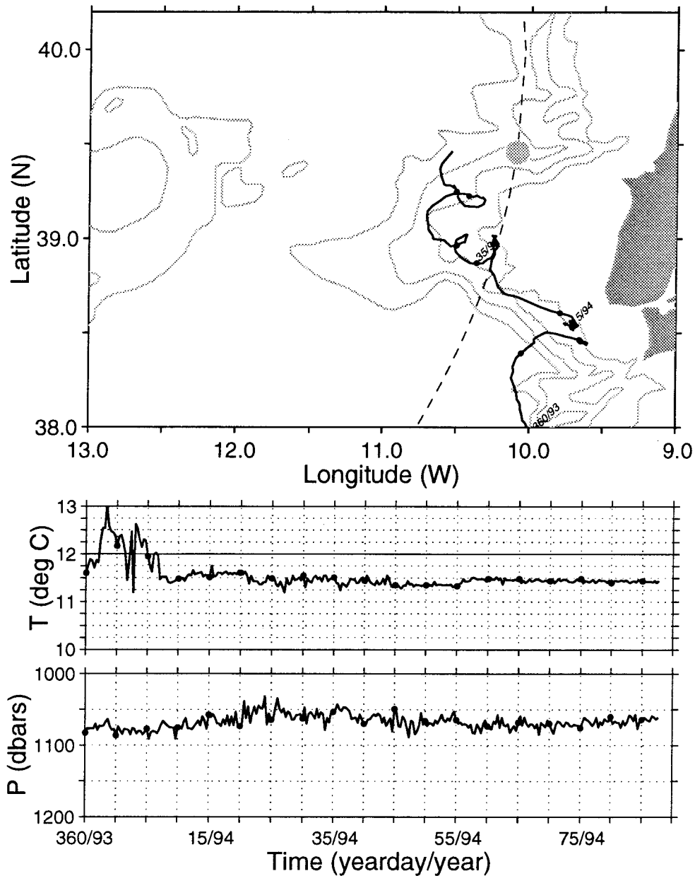
FIG. 14. As in Fig. 13 except for am138 (K0407) launched on 28 September 1993, yearday 240/93. Dashed curve shows range from sound source as described in the text. Shaded circle indicates hypothetical meddy position on yearday 57/94.
