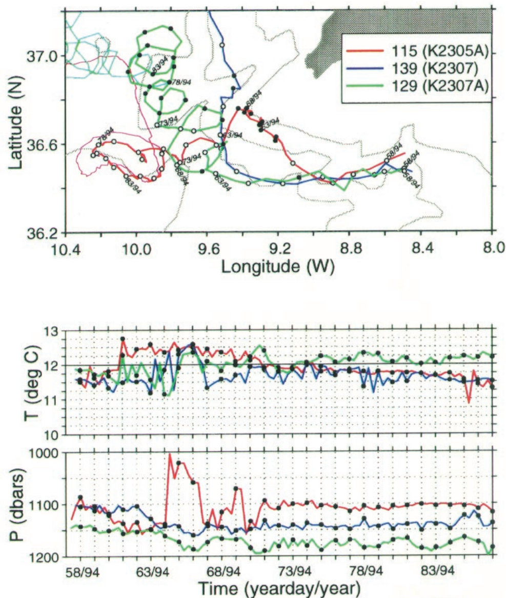
FIG. 9. Event 5: As in Fig. 6 but for am115 (K2305A, red), am139 (K2307, blue), and am129 (K2307A, green) launched on 26 February 1994, yearday 57/94. Note change in scales in upper panel compared to previous figures.
