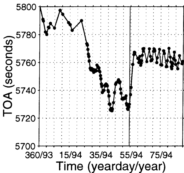
FIG. 16. Time series of time of arrival (TOA) from sound source located at 40^{\circ}\text{N} , 15^{\circ}\text{W} as observed by am138. Dots indicate actual observations. Vertical line at year/day 54/94 indicates time of last position (see text). TOA is measured in elapsed seconds from 0000 UTC.
