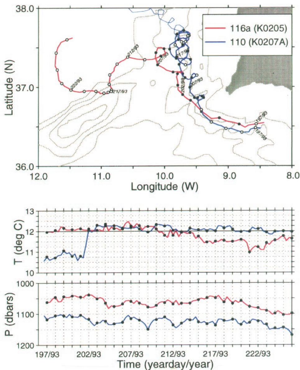
FIG. 7. Events 2 and 3: Same as in Fig. 6 but for am116a (K0205, red) and am110 (K0207A, blue) launched on 15 July 1993, yearday 196/93. Only the first 30 days of temperature and pressure data for am110, corresponding to highlighted part of the track in the upper panel, are shown.
