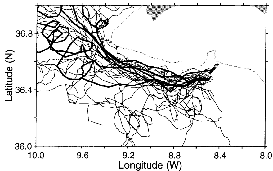
FIG. 19. Superposition of the first 30 days of tracks for 32 floats deployed at the level of the lower core of the Mediterranean Undercurrent ( P > 1000 dbars). Tracks of the first five meddy floats are highlighted and the 1000-m isobath is also shown for reference.
