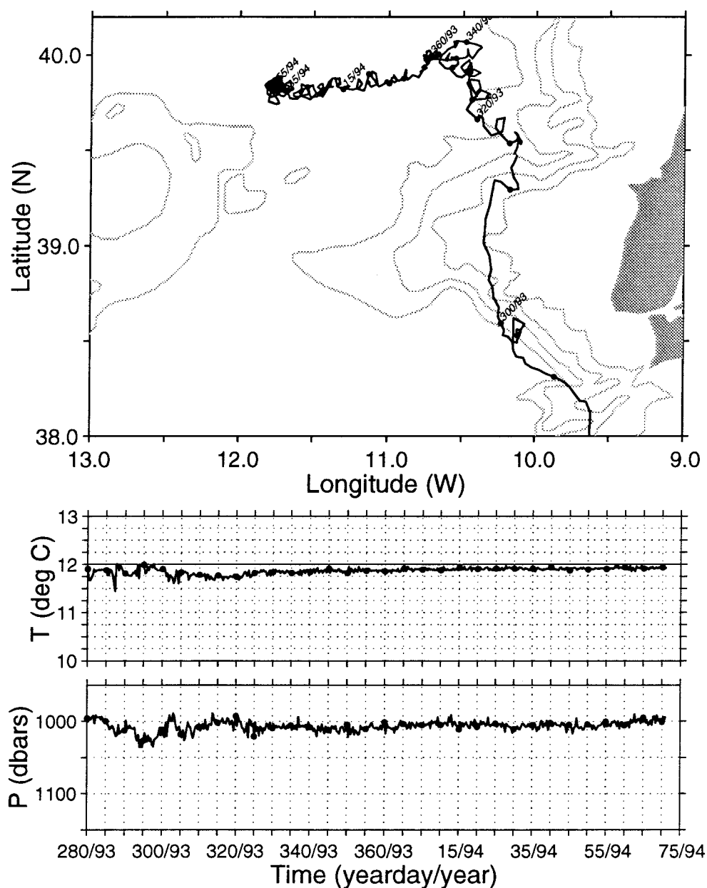
FIG. 13. Portion of trajectory of am118 (k0506) launched on 4 September 1993 yearday 247/93. Dots indicate position (but not temperature) at 5-day intervals and the 1000–4000-m isobaths are also plotted. Temperature and pressure records along the float track are shown in lower panels.
