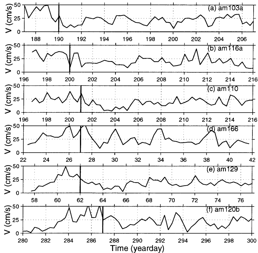
FIG. 12. Time series of float speed for six meddy floats during the first 20 days of each track. Heavy vertical lines indicate approximately when anticyclonic looping began.
