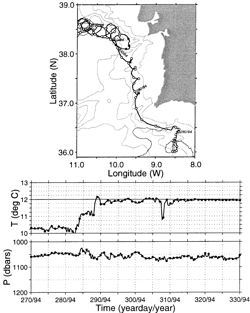
FIG. 10. Event 6: As in Fig. 6 but for am120b (K2406) launched on 5 March 1994, yearday 64/94. Highlighted track and temperature and pressure shown for 60 days starting on yearday 270/94.
