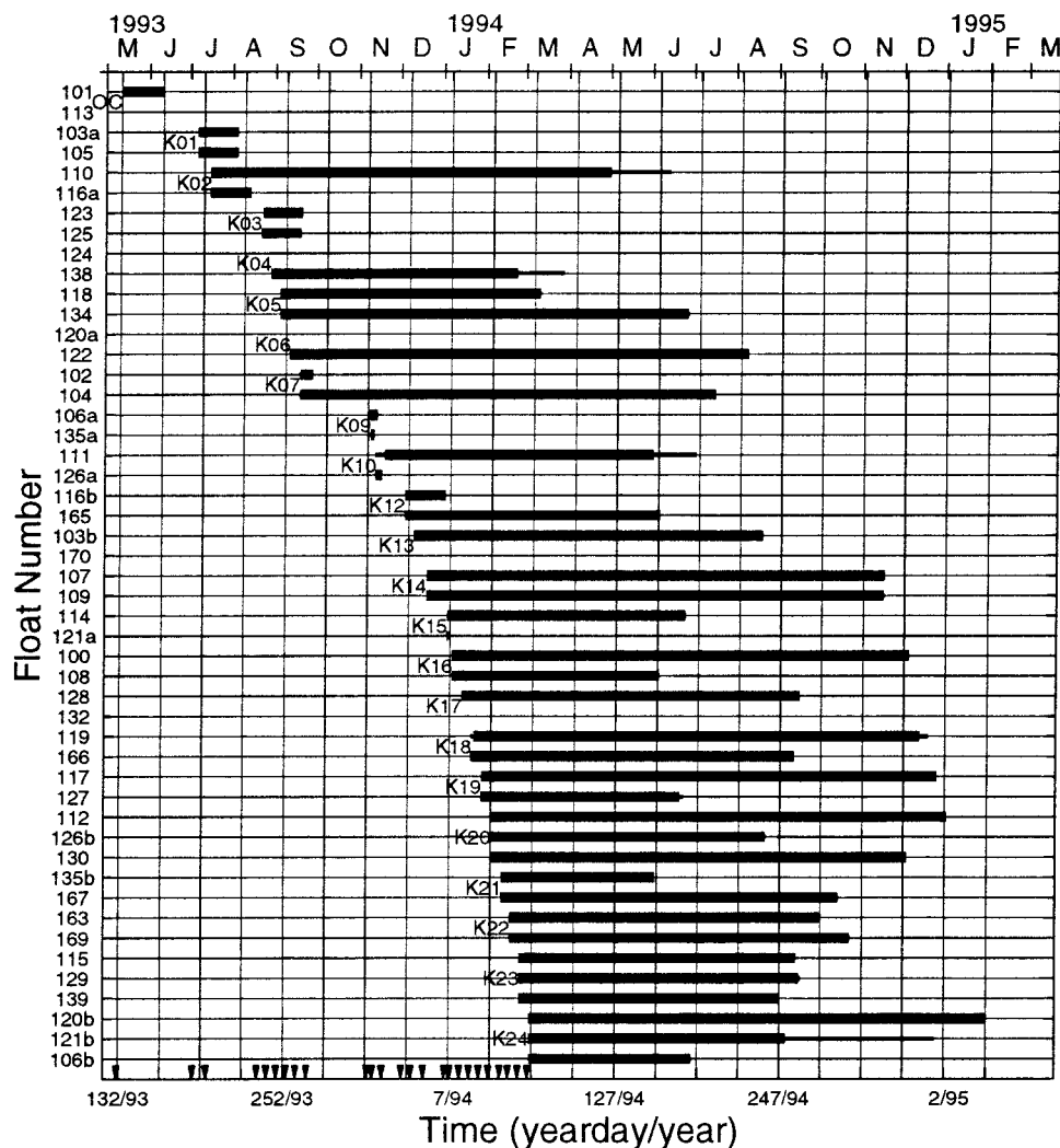
FIG. 4. Time line of R/V Oceanus and Kialoa II cruises and float launchings during AMUSE. Time is indicated in year/day and year (94 = 1994) along the bottom axis and by month and year along the top axis. The inverted triangles along the bottom axis show the times of the one R/V Oceanus cruise and 24 Kialoa II cruises. The heavy horizontal lines indicate the duration of each float mission (line is slightly thinner when only temperature and pressure data were obtained), and the labels (e.g., K01) refer to the cruise on which each set of floats was deployed.
