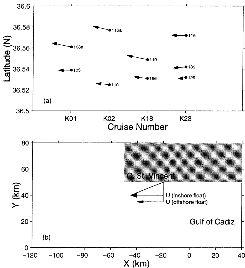
FIG. 21. (a) Mean velocity vectors measured over the first three days after the launch for floats deployed on K01, K02, K18, and K23 showing the relative speed of floats launched at different cross-slope positions. (b) Schematic view of the southwestern corner of the Iberian Peninsula and estimation of horizontal shear in undercurrent from float velocity observations. See text for explanation.
