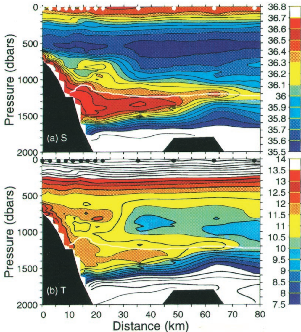
FIG. 3. Vertical distributions of (a) salinity (contour interval = 0.1) and (b) temperature (contour interval = 0.5^{\circ}\text{C} ) along section indicated in Fig. 2. Northern end of the section is to the left. The station locations are plotted as dots along the top axis. The heavier white line shows the depth of the 32.25\sigma_t density surface along the section.
