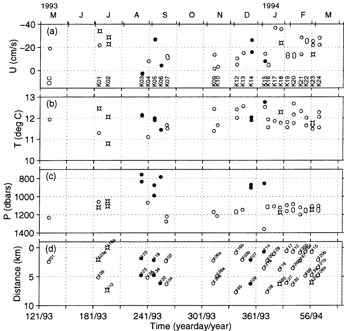
FIG. 18. (a) Time series of average zonal velocity measured by each float during first three days after launch as a function of time. Unfilled circles indicate floats near the level of the lower core ( P > 1000 dbars) and x's mark the five floats that ended up in meddies; (b) 3-day mean temperature; (c) 3-day mean pressure; and (d) launch position measured as distance from northernmost float launch site, 05. Float numbers are also indicated. The + 's along the top axis of (a) indicate month boundaries.
