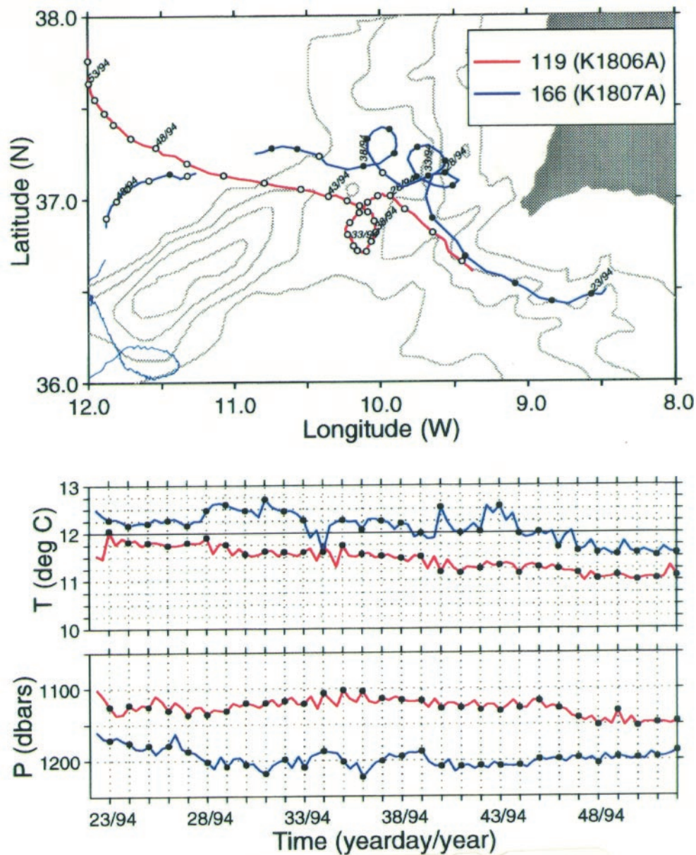
FIG. 8. Event 4: As in Fig. 6 but for am119 (K1806A, red) and am166 (K1807A, blue) launched on 22 January 1994, yearday 22/94. Note that the first few days of am119's trajectory are missing due to poor acoustics.
