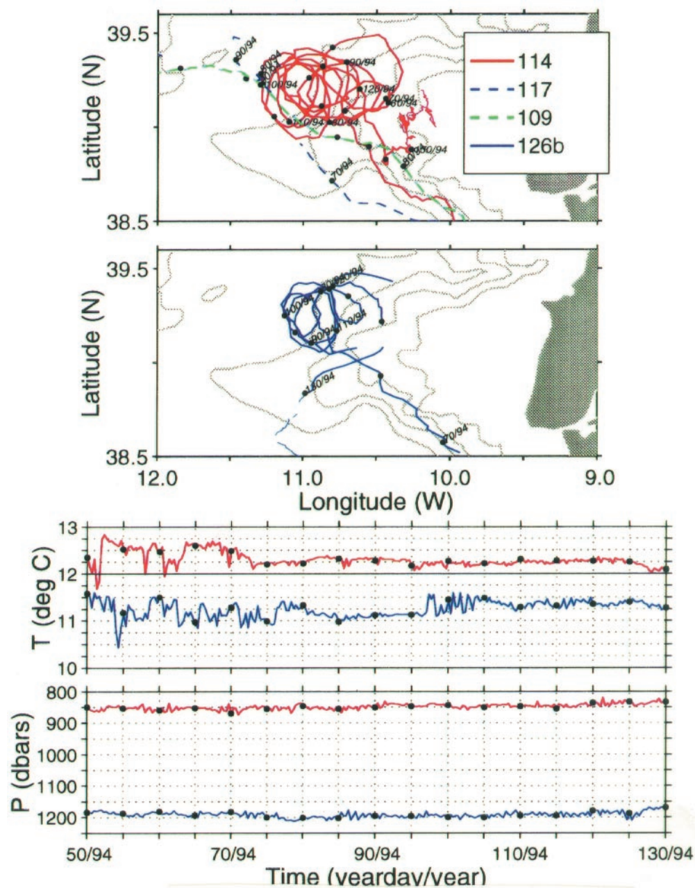
FIG. 15. Trajectories of am114 (K1505A, red), am117 (K1905A, dashed blue), and am109 (K1407A, dashed green) are shown in the upper panel, highlighted during time period 50/94 through 130/94. Dots are plotted every 5 days along tracks. Am126b (K2006A, blue) is shown in second panel during same time period. Temperature and pressure along float tracks am114 (red) and am126b (solid blue) only are shown in lower panels.
