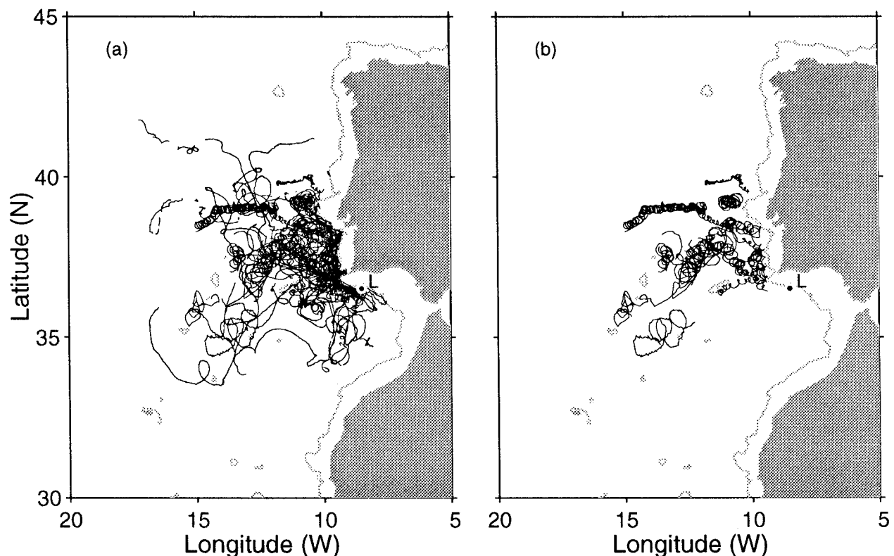
FIG. 5. (a) Spaghetti diagram of all 44 floats that returned useful data during AMUSE; (b) tracks of 14 floats that observed meddies. The 1000-m isobath is indicated by a gray line, and the float launch site is labeled with an "L."
