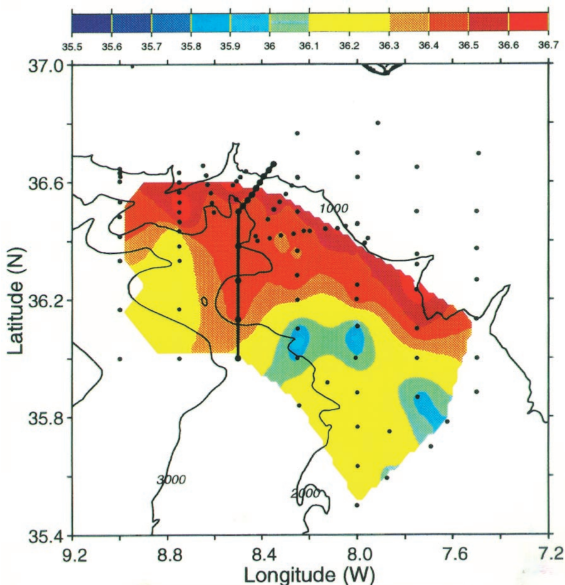
FIG. 2. Salinity on the 32.25 \sigma_t density surface in the western Gulf of Cadiz during the preliminary CTD survey conducted in May 1993 aboard R/V Oceanus . The shading interval is 0.1. Station positions are indicated by dots. Section shown in Fig. 3 is indicated by bent line. Thin underlining contours indicate water depth in 1000-m intervals.
