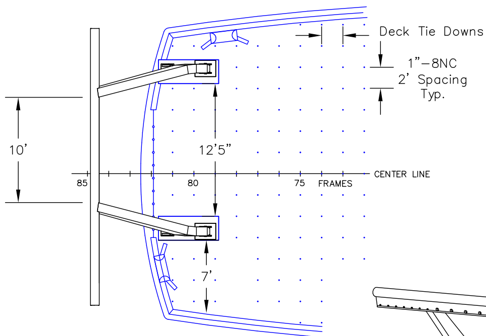
Plan View of Stern
