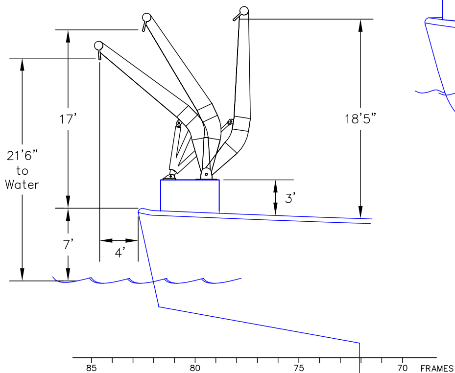
Profile of Stern
