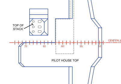
05 DECK, R/V ATLANTIS
