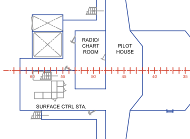
04 DECK, R/V ATLANTIS
