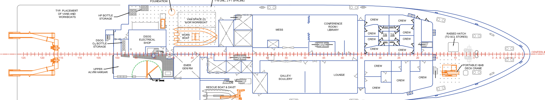
01 DECK, R/V ATLANTIS
