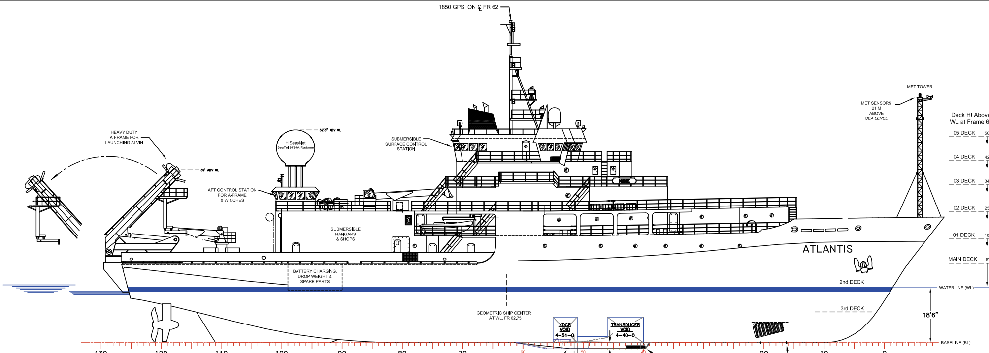
COMPOSITE PROFILE, R/V ATLANTIS
