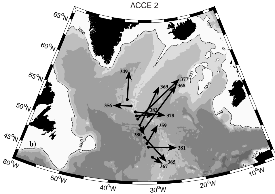
Figure 1. RAFOS float displacement vectors, separated by cruise. Vectors are labeled with float number at the arrowhead. Dots mark the launch positions, and arrowheads the surface positions. The 1000-meter isobath is drawn; bathymetry is shaded in 1000-meter intervals. a) ACCE 1, b) ACCE 2, c) ACCE 3: western deployments, and d) ACCE 3: eastern deployments. Composite vector diagram including all floats is shown in the front cover figure.
