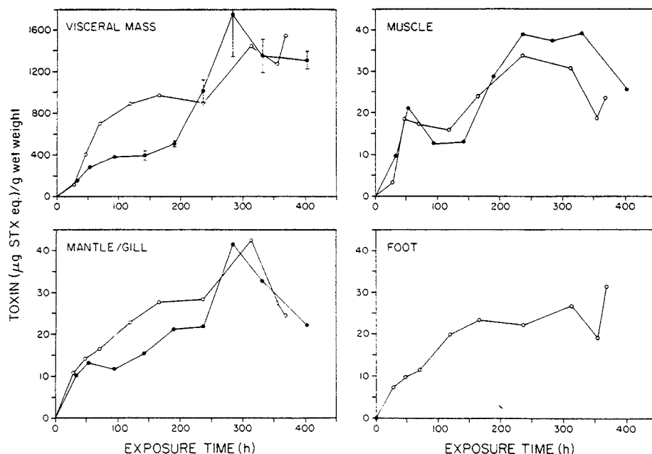
Fig. 5. Mytilus edulis . Patterns of PSP toxin accumulation ( \mu\text{g STX eq. [g wet tissue wt]}^{-1} ) in mussel tissues (Series I and II as in Fig. 4). Toxin was determined from pooled samples ( n = 4 ). Where error bars are shown, these represent 95% CI of 2 samples, each with pooled tissues from 2 individuals
