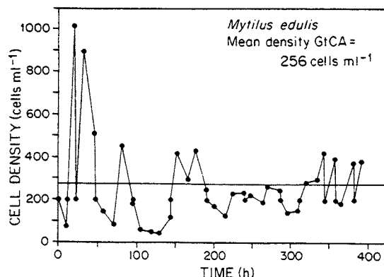
Fig. 3. Concentration of Alexandrium fundyense in the experimental tank. Horizontal line indicates time-weighted mean cell density over the 17 d toxin uptake experiment
