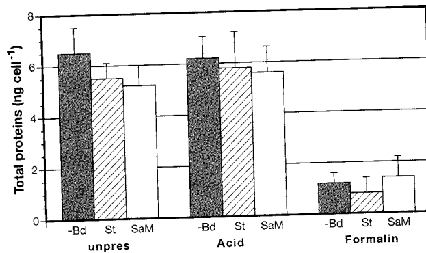
Fig. 6. Total amount of protein per cell in unpreserved and preserved cultured Alexandrium fundyense cells after isolation using the indirect technique. unpres: no preservative used; -Bd: control cells without bead treatment; St: cells after bead isolation with M-280 Streptavidin beads; SaM: cells after bead isolation with M-280 SaM beads. Error bars represent \pm 1 SD for each treatment
