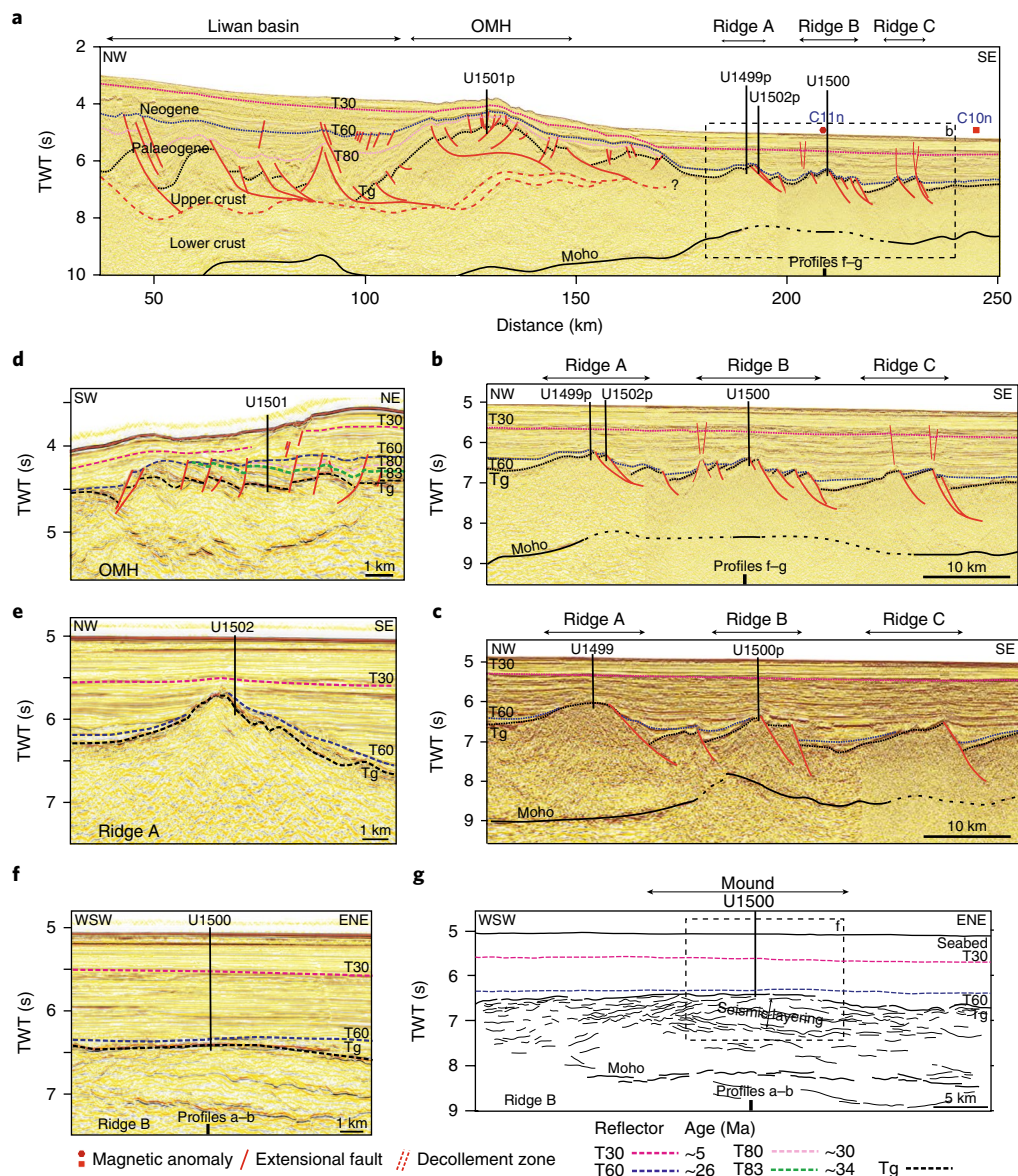
Fig. 2 | Interpreted seismic sections. For location of sections see Fig. 1. Drill sites marked with 'p' are projected. a , Regional seismic profile crossing the northern SCS margin. b, c , Expanded views of Ridges A, B and C, emphasizing their lateral continuity. d–f , Seismic sections across the drilling sites. g , Line drawing from a strike line across Ridge B showing a mound-like structure below Site U1500, suggesting that slightly younger volcanic strata may subcrop elsewhere along the ridge. Seismic data are taken and modified from refs 16,51 . The Chinese National Offshore Oil and Gas Company (CNOOC) convention for naming seismic stratigraphic unconformities 55,56 has been adapted. Regional seismic stratigraphic unconformities T30–T83 with ages are obtained from IODP drill cores. The T60 unconformity reflects some late, post rift deformation of minimal extension, possibly related to lower crustal flow 25 . Tg: acoustic basement does not represent a time line or specific stratigraphic relationships of lithologies (Fig. 3). Black line: Moho reflector (verified directly below Ridge B by wide-angle data 28 ).
