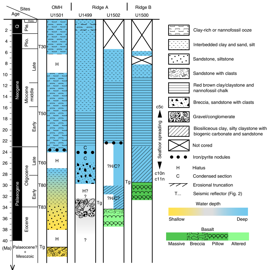
Fig. 3 | Summary chart of drilling results. Ages based on core samples analysed for calcareous nannofossils, foraminifers, diatoms and ostracods. Lithostratigraphy is from detailed core descriptions 29,32–34 following the GTS12 48 geological timescale.
