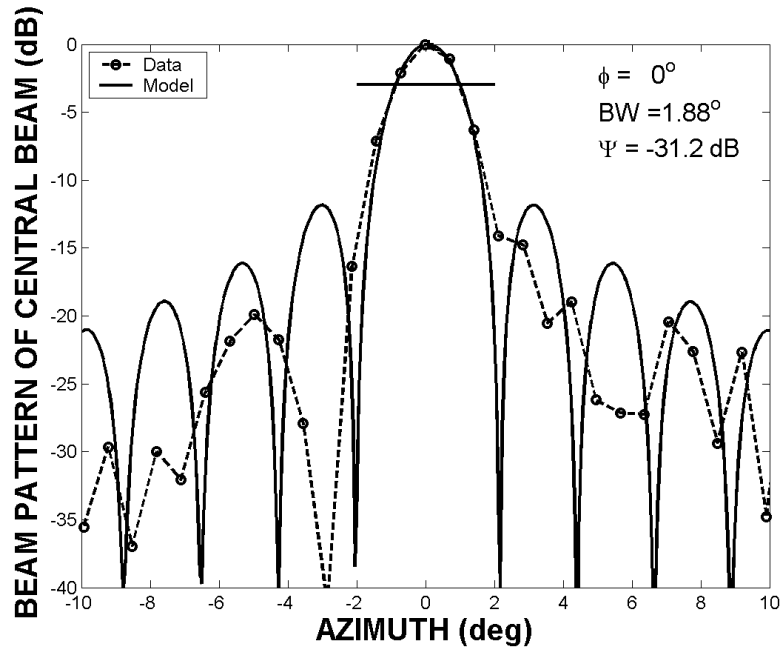
Figure 3. Beampattern of beam at 0^\circ . The 3-dB beam width is 1.88^\circ and the equivalent beam angle in log-scale is -31.2 dB.
