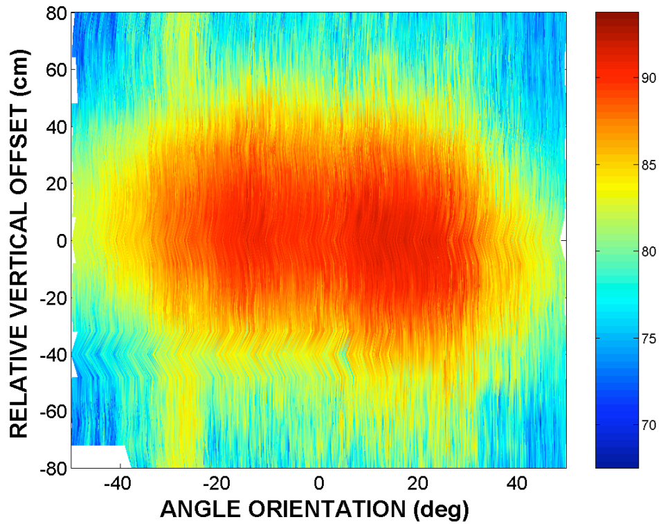
Figure 2. 2-D directivity pattern of SM2000/90 kHz multibeam sonar, measured at 23 m range.
