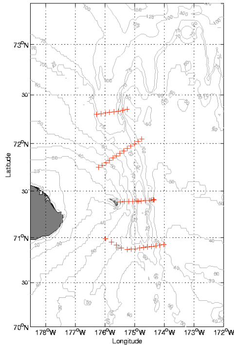
Figure 1: (a) Bottom topography of the Chukchi Sea showing the two canyons that help steer the flow from Bering Strait. The depth is in meters (key on the right). (b) Hydrographic stations (red crosses) comprising the RUSALCA Herald Canyon survey. The survey took roughly three days to complete.
