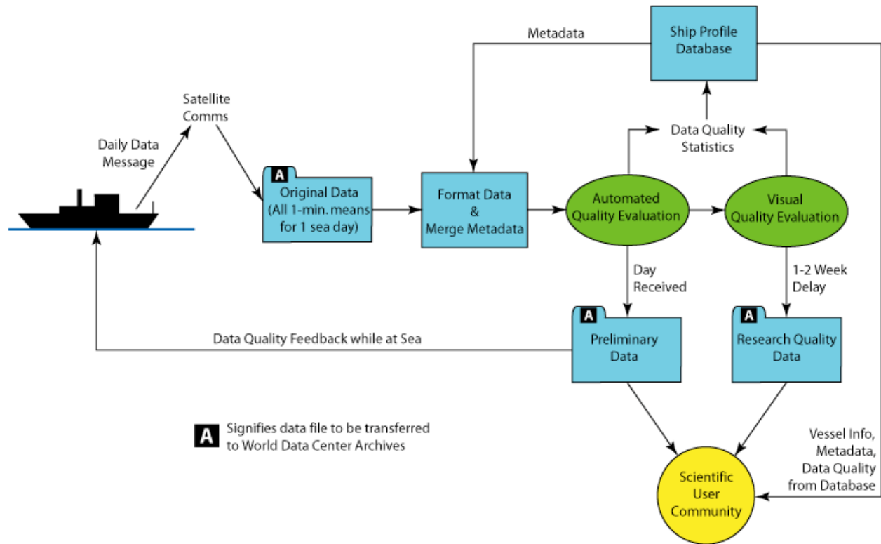
Fig. 1: SAMOS data flow to be tested during the 2005 pilot project with WHOI and SIO.
