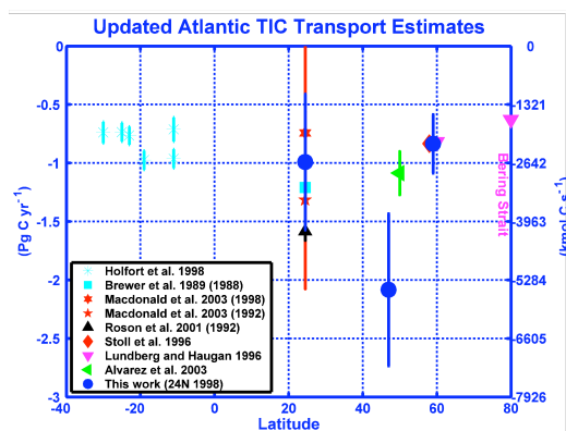
Figure 2: Atlantic TIC transport estimates as a function of latitude from various independent studies, including the North Atlantic model discussed here. Net flux through Bering Strait and the Arctic are included in all the estimates.
