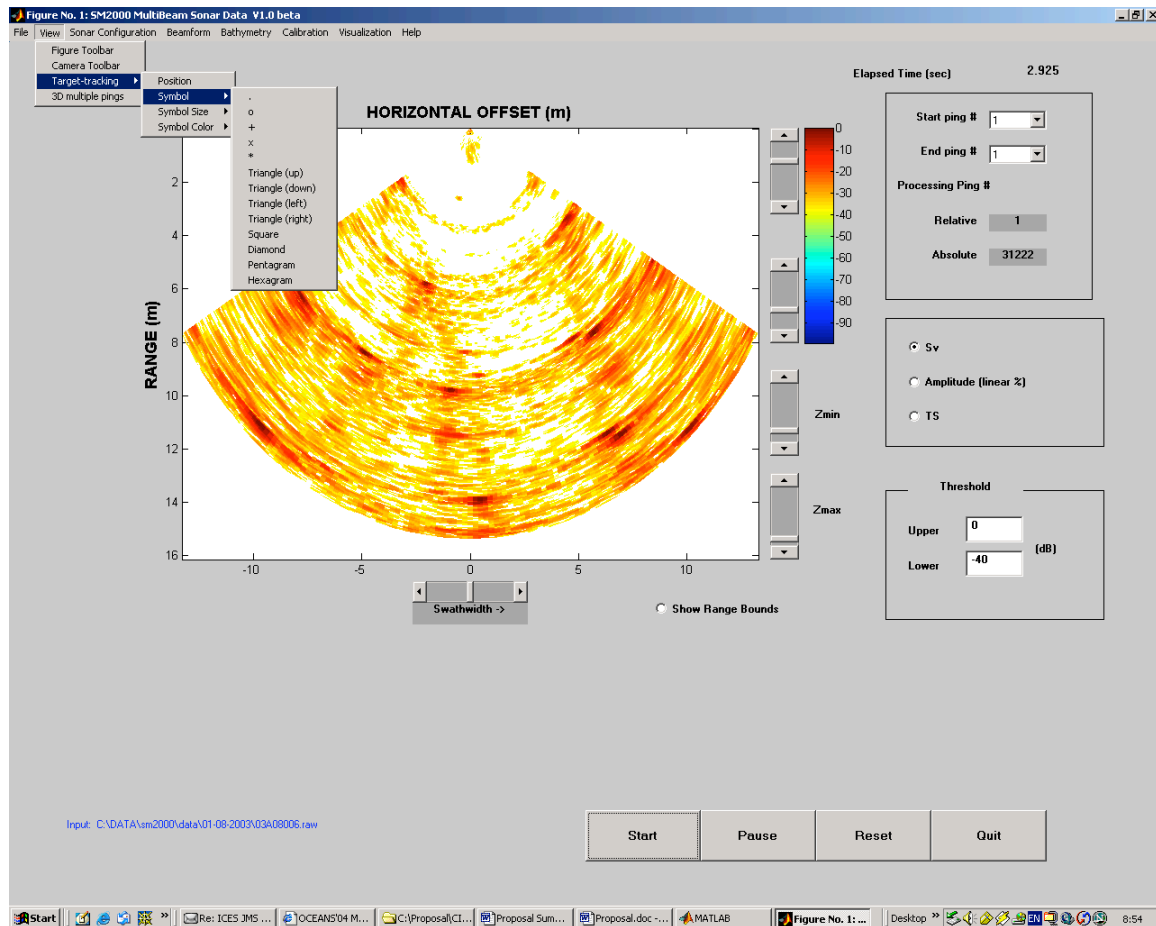
Figure 6. Graphic User Interface (GUI) of the Quantitative Multi-Beam Sonar Processing (QMBSP) software. Dark spots represents echoes from the discrete targets.
