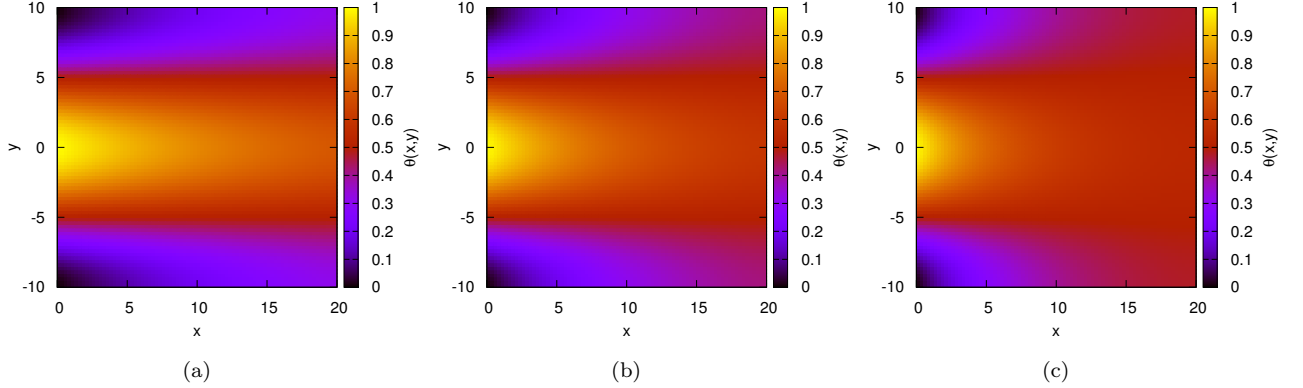
Figure 6: Three different 2D scalar fields resulting from the solution of the advection-diffusion equation of Eq.(3) with a flow field moving from left to right with a constant flow magnitude of unity. Figure 6a shows the solution \theta(x,y) for a diffusivity of 0.5, Figure 6b shows the solution for a diffusivity of 1.0, and Figure 6c shows the solution for a diffusivity of 2.0. The quoted values for diffusivity refer to the numerical values used for both \kappa_x and \kappa_y in Eq.(3). For each case, there is a Dirichlet boundary condition at the left domain boundary that specifies a time-invariant concentration there. The rest of the scalar field is the steady-state solution of the advection-diffusion equation.
