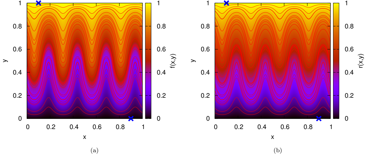
Figure 5: A simple analytic test case that illustrates the potential of the flow-based interpolation method. Figure 5a shows an oscillating scalar field f(x,y) whose isocontours are streamlines of the associated flow field. The flow-based scattered data interpolation method produces an adequate reconstruction r(x,y) of the oscillating scalar field based on knowledge of the flow field and only two samples of the scalar field (denoted by the blue markers), as can be seen in Figure 5b.
