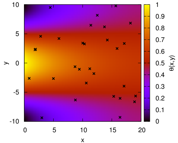
Figure 7: A 2D scalar field \theta(x, y) in the presence of a left-to-right flow field, constructed using the advection-diffusion model of Eq.(3), with 30 scattered samples indicated.
