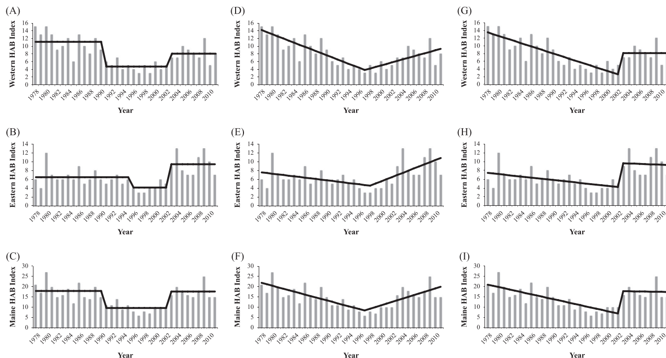
Fig. 7. Mean-shift (A–C), two-phase (D–F), and pulse-decline (G–I) models fitted to time series of the HAB Index for eastern and western Gulf of Maine separately, and together.
