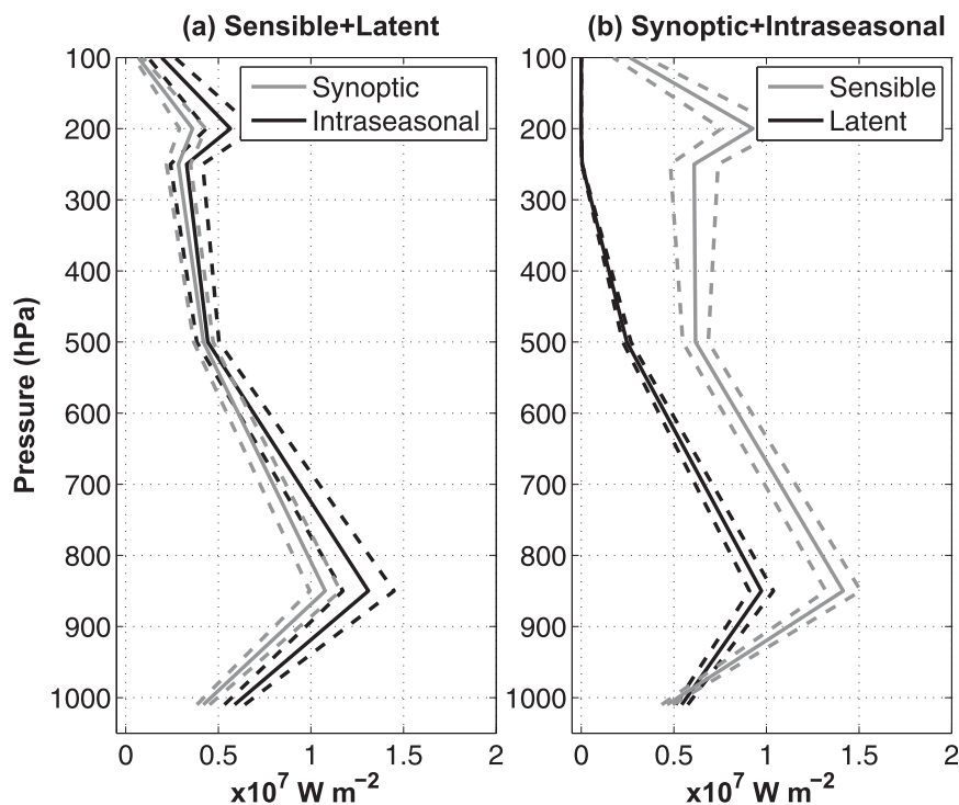
FIG. 3. Vertical profiles of winter (JFM) meridional heat fluxes by transient eddies averaged over the zonal band between 30^{\circ} and 50^{\circ}\text{N} for (a) sensible + latent components and (b) synoptic + intraseasonal bands. The thick lines are for the 31-yr mean, and the dashed lines indicate one standard deviation ranges.
