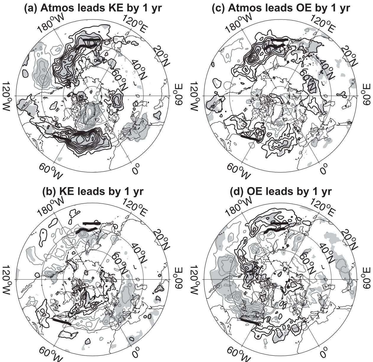
FIG. 14. Lag regressions of winter (JFM) vertically integrated meridional heat flux by synoptic transient eddies on the winter (a),(b) KEI and (c),(d) OEI. Positive (negative) regression coefficients are contoured with black (gray) lines. Zero contours are suppressed. Contour intervals are 0.2 \times 10^7 \text{ W m}^{-1} , and shadings indicate regression values significant at 90%. The mean positions of the GS and OE are indicated by thick black curves, and KE is indicated by thick dashed curve.
