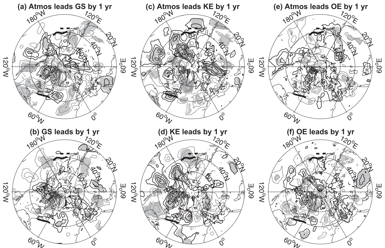
FIG. 15. Lag regressions of winter (JFM) vertically integrated meridional heat flux by intraseasonal transient eddies on the winter (a), (b) GSI, (c), (d) KEI, and (e), (f) OEI. Positive (negative) regression coefficients are contoured with black (gray) lines. Zero contours are suppressed. Contour intervals are 0.5 \times 10^7 \text{ W m}^{-1} , and shadings indicate regression values significant at 90%. The mean positions of the GS and OE are indicated by thick black curves, and KE is indicated by thick dashed curve.
