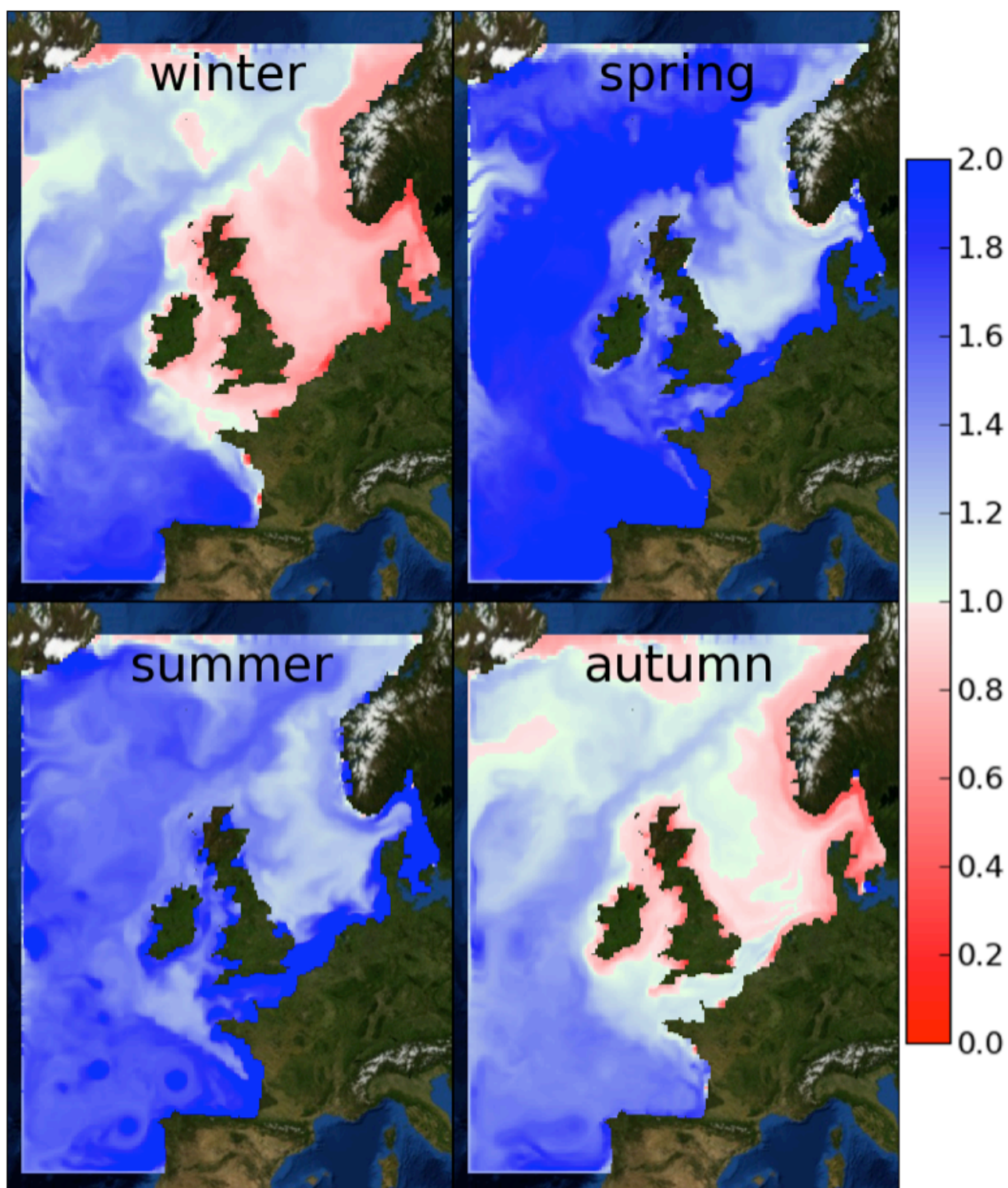
Figure 1: Seasonal snapshots of aragonite saturation state for the surface layer of the NW European shelf seas at p\text{CO}_2 atmosphere = 1000 ppm. Apart from p\text{CO}_{2a} , all other forcing fields are as for the year 2000.
