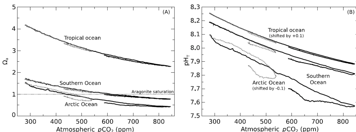
Figure 1: Saturation state with respect to aragonite and pH T in surface water of three regions as a function of atmospheric CO 2 . Results are from emission commitment scenarios with high (solid) or medium (dashed) 21st century emissions and no emissions after 2100. The relation between atmospheric CO 2 and saturation state and pH T shows almost no path dependency in the tropical ocean and Southern Ocean. Some path dependency is found in the Arctic Ocean, with lower values in surface saturation and pH T for a given CO 2 concentration simulated after the peak in atmospheric CO 2 . Note that the pH T – CO 2 curves are shifted by +0.1 pH units for the tropical region and by –0.1 pH units for the Arctic region for clarity.
