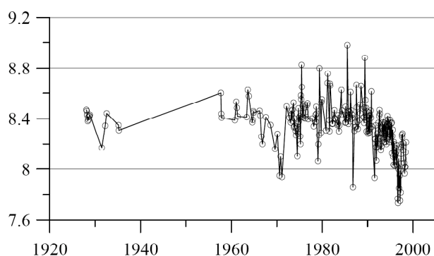
Figure 1: Time series of monthly pH at the surface.
