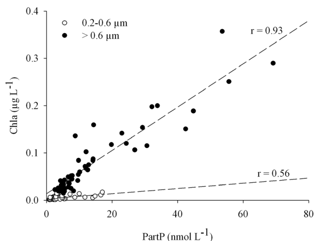
Fig. 3. Relations between Chlorophyll a (Chla) and particulate phosphate (PartP) at depth corresponding to a range of PAR levels between 50% and 15%, for two size fractions: 0.2–0.6 µm and >0.6 µm.
