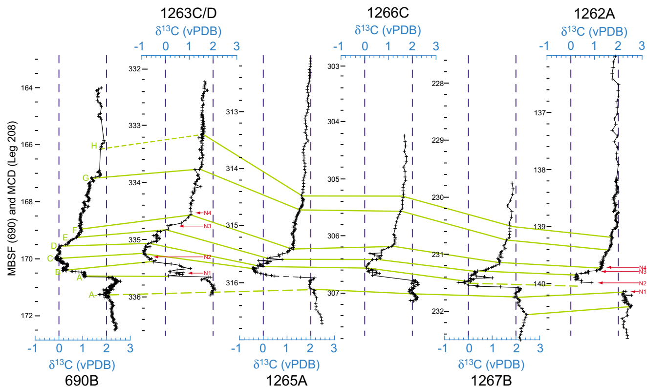
Fig. 2. Bulk sediment carbon isotope records for holes 1262A, 1263C/D, 1265A, 1266C, and 1267B plotted versus MCD. Also plotted are nannofossil horizons (N1 to N4, arrows in red) for holes 1262B and 1263C/D (20). Data for ODP site 690 (22) are plotted to the far left
